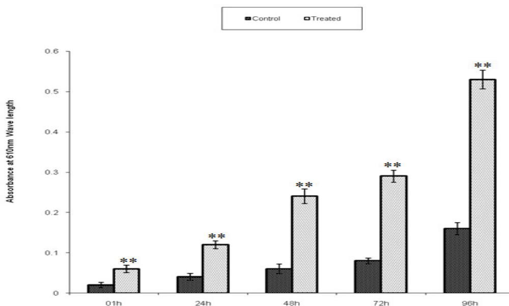
Fig 1. Optical density of test water at 610_{\text{nm}} wavelength for different times on exposure to sub lethal concentration ( 27.27 \text{ mg L}^{-1} , 75% of 96\text{h LC}_{50} ) of dimethoate. Values are mean \pm SD of eight animals. Asterisks indicate insignificant (*) and significant (**) differences at P < 0.0001 level from control.
