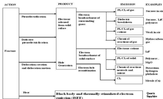
Fig 1. Schematic diagram for the mechanisms of fracto-ML.
