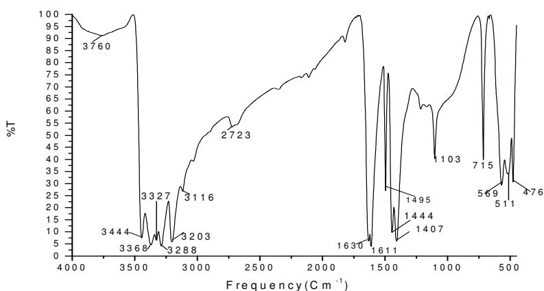
Fig 3. FTIR spectra of ZTTC crystal
