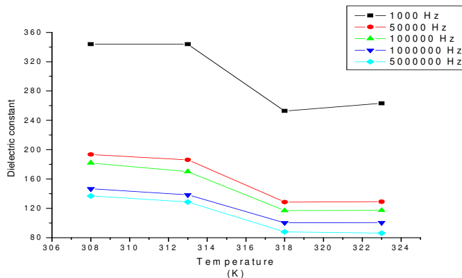
Fig 7. Temperature dependence of dielectric constant for ZTTC single crystal
