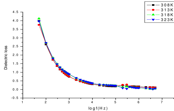
Fig 6 . Variation of dielectric loss of ZTTC with log frequency.
