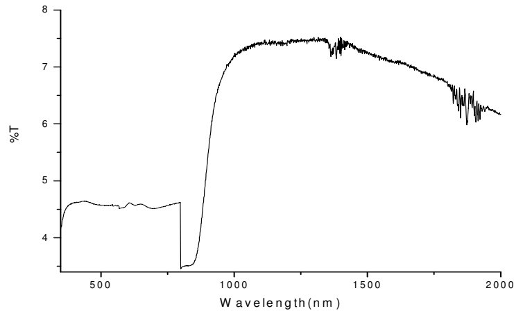
Fig 4 . Transmission spectrum of ZTTC.
