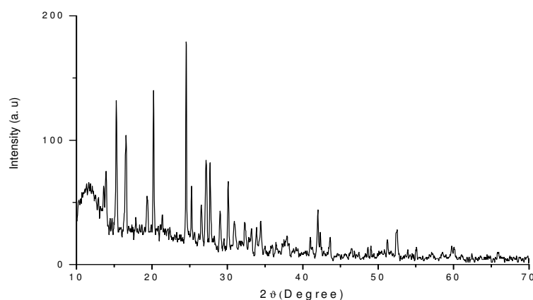
Fig 2. Powder X-ray diffraction pattern.
