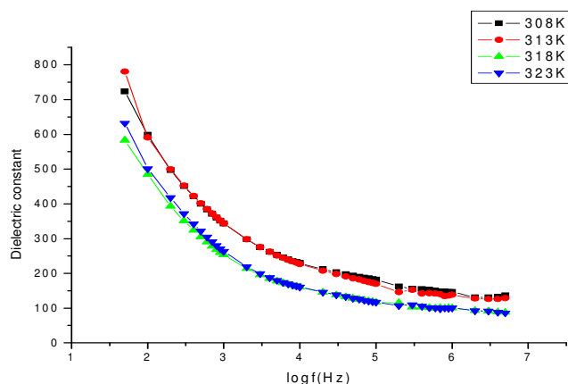
Fig 5 . Variation of dielectric constant of ZTTC with log frequency.
