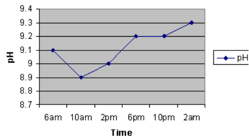
Fig. 3: Diurnal variation of pH
