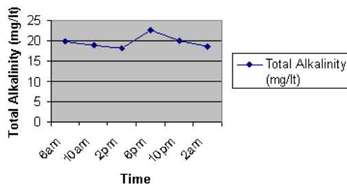
Fig. 7: Diurnal variation of total alkalinity (mg/l)
