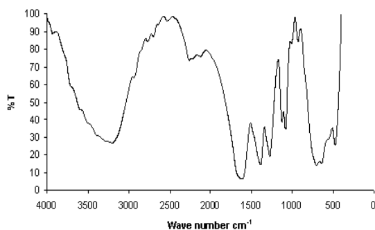
Fig.3 FTIR spectrum of SBT single crystals
