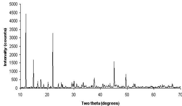
Fig.2 Powder X-ray diffractogram of SBT crystals
