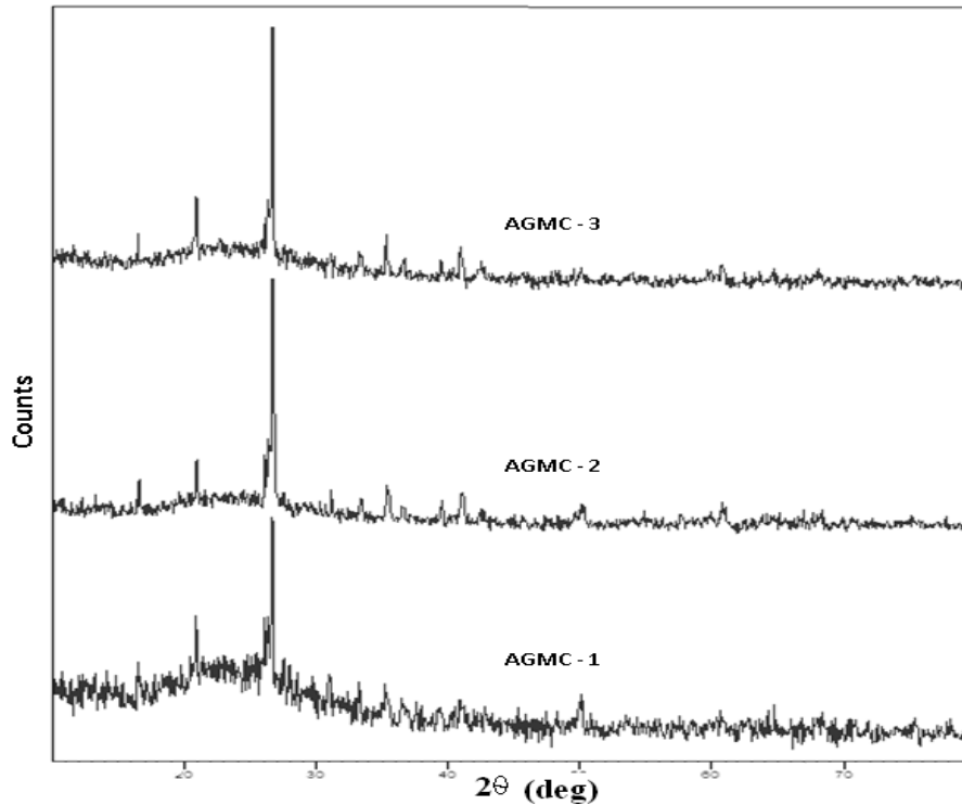
Fig.3 X- ray diffraction pattern of Alagankulam celadon sherds
