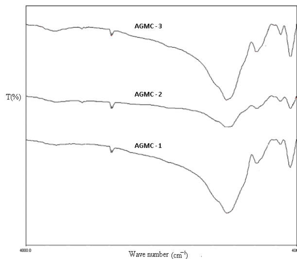
Fig.2 FT-IR spectra of Alagankulam celadon sherds in the as-received state
