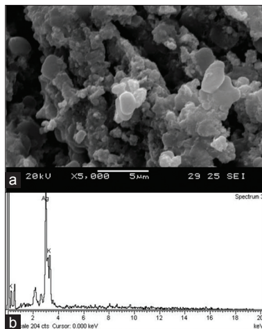
Figure 4: Silver nanoparticles biosynthesized using the Sida acuta leaf extract: (a) Scanning electron micrograph (5000×); (b) EDX spectrum showing chemical composition
