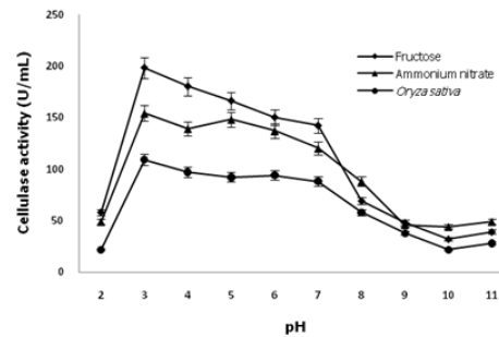
Fig. 5. Effect of initial pH value on cellulase activity
