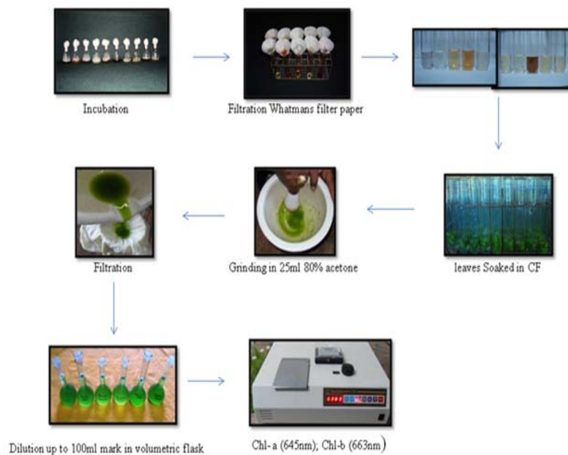
Fig1: Estimation of Chlorophyll from Spinach
