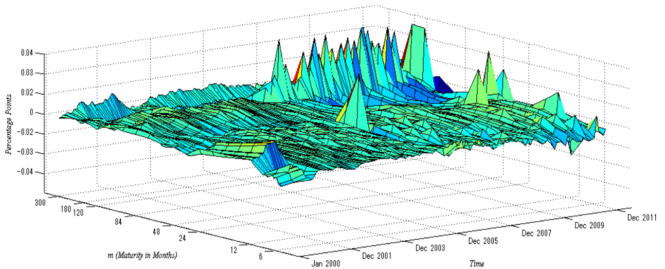
Figure 5: Nelson–Siegel Model based Yield Curves Residuals, 2000:01–2011:12 for Time-varying \tau .
