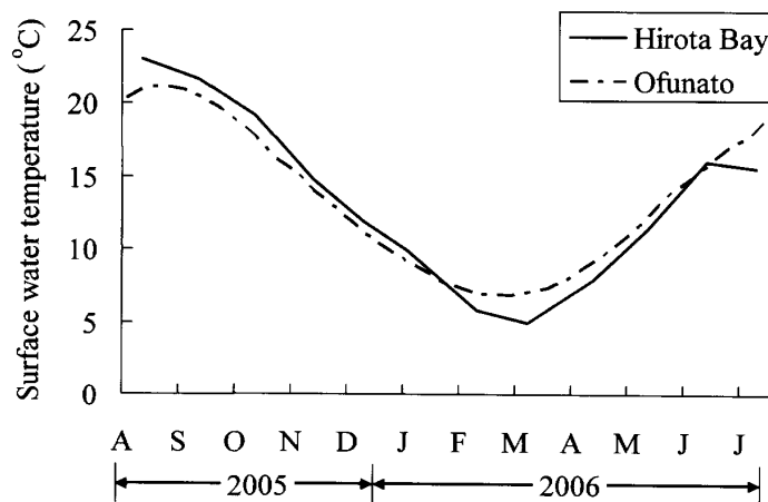
FIG. 2. Surface water temperature in Hirota Bay from August 2005 to July 2006 and monthly average water temperature for 27 years (1980–2006) at Ofunato.
