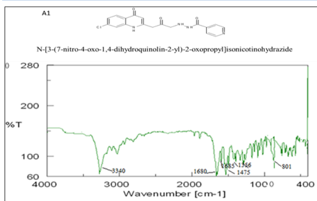
Figure 1. IR Spectra of A 1
