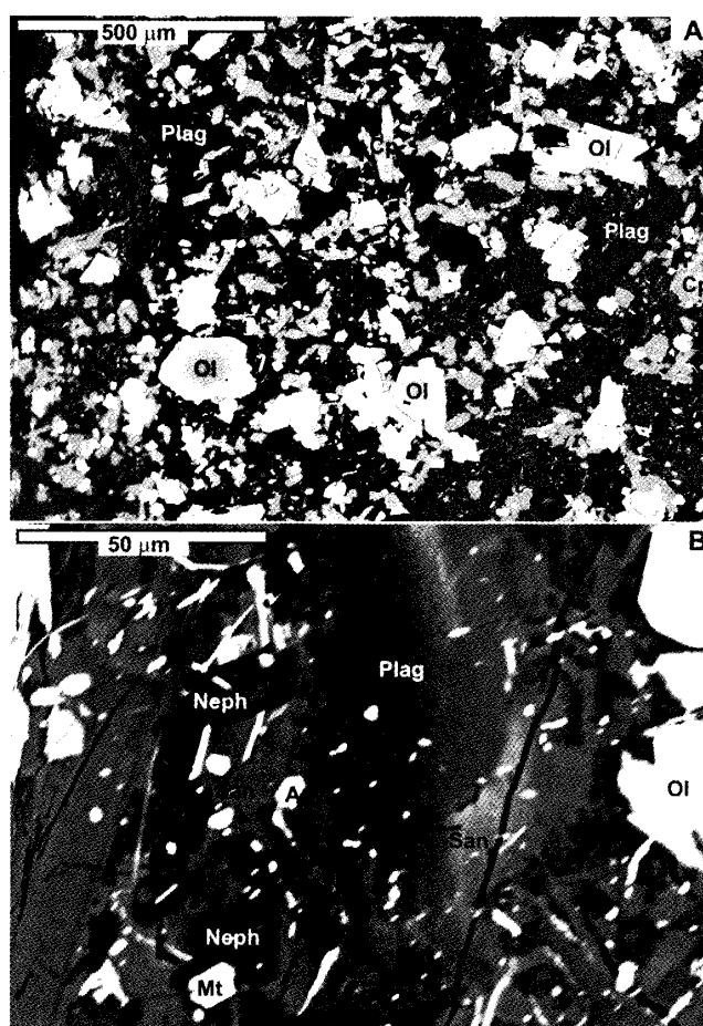
Figure 2. Back-scattered electron image (BEI) of host basanite from Dzhilinda River. A, texture of groundmass and phenocrysts. B, coexistence of albite (Ab), plagioclase (Plag), and nepheline (Neph). Ol, olivine, Cp, clinopyroxene, Mt, Ti-magnetite, Ap, apatite.
