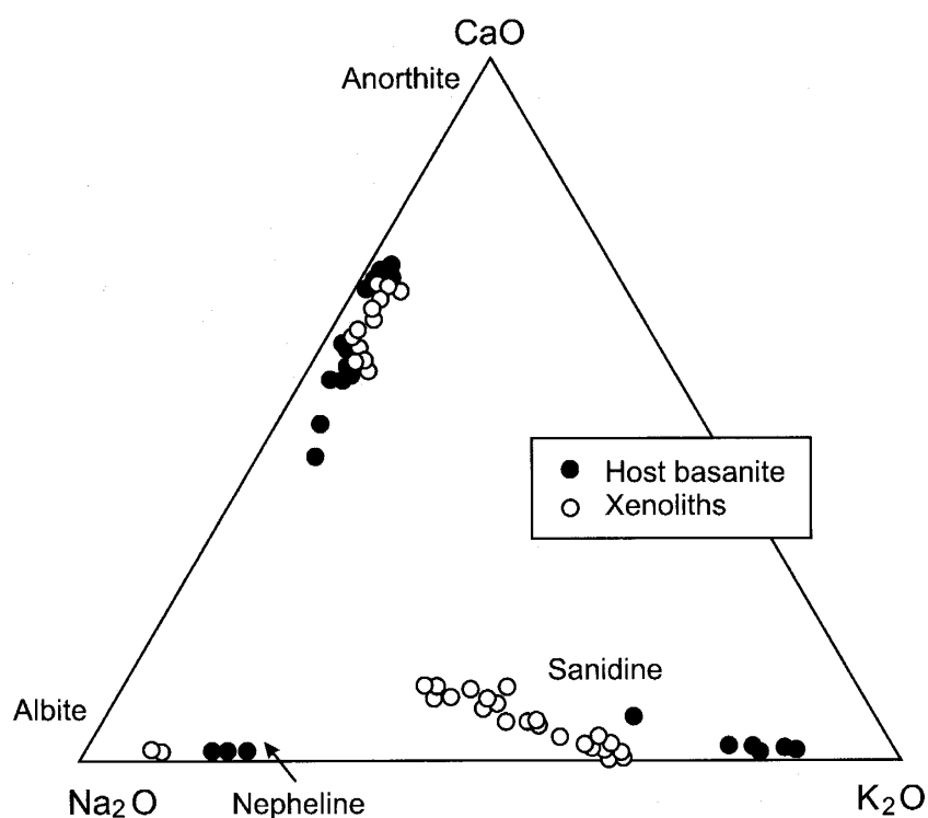
Figure 6. Feldspar and feldspathoid compositions from microlites in Ti-rich xenoliths in the diagram Na 2 O-CaO-K 2 O.
