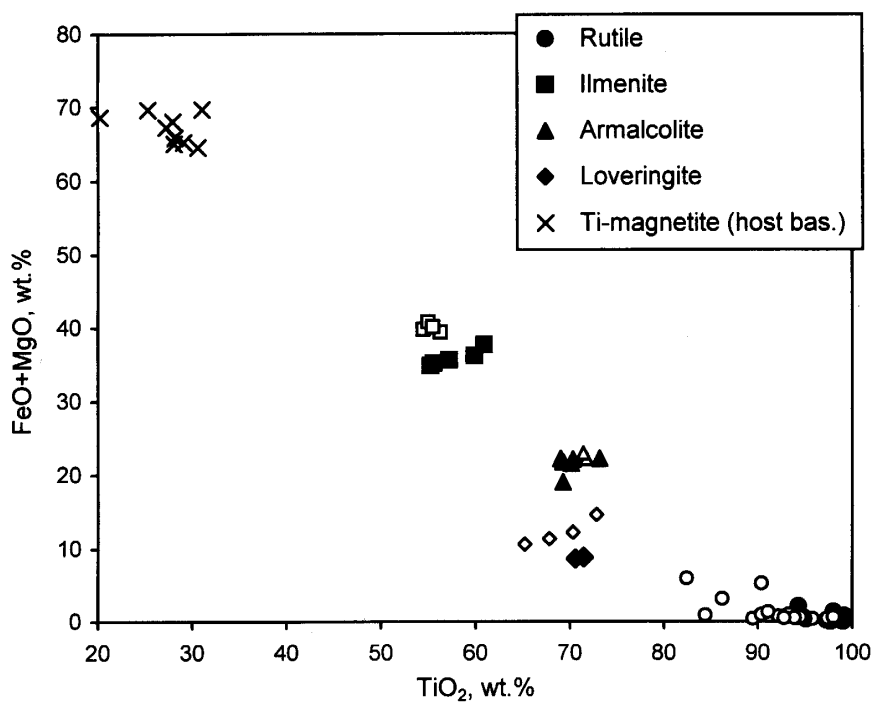
Figure 7. Compositional variations of Ti-oxide minerals in Ti-rich peridotite xenoliths and host basanite of Dzhilinda River. Open symbols, data from Kalfoun et al. (2002) for minerals from peridotite xenoliths of Sikhote-Alin (Russian Far East).
