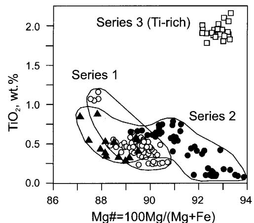
Figure 1. Composition of clinopyroxenes from the Dzhilinda basanites.
