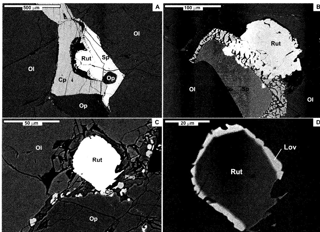
Figure 4. BEI of interstitial rutile in Ti-rich xenoliths from Dzhilinda River. A-B, Sample DJ-1, large rutile grains in close intergrowth with spinel. Note recrystallization of spinel and rutile by impregnation of basanite melt. C-D, Sample DY-8A, rutile grain in the melt pocket, (D, reaction rim of loweringite (Lov) at the rutile grain (see Table 3). See Fig. 2-3 for abbreviations.
