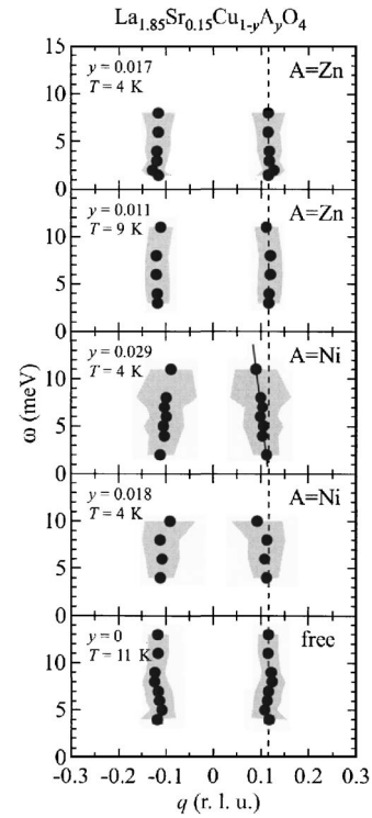
FIG. 11. Spin excitations for y=0 , \text{La}_{1.85}\text{Sr}_{0.15}\text{Cu}_{1-y}\text{Zn}_y\text{O}_4 (Zn: y=0.011, 0.017 ) and \text{La}_{1.85}\text{Sr}_{0.15}\text{Cu}_{1-y}\text{Ni}_y\text{O}_4 (Ni: y=0.018, 0.029 ), at low temperature. q denotes the propagation vector of spin correlation; q=0 means the magnetic zone center Q=(0.5, 0.5, 0) . Solid circles and shaded regions represent the peak position and FWHM of incommensurate magnetic signals estimated from curve fitting. Dashed lines show a mean value of peak positions for the impurity-free sample. A solid line indicates a guide to the eye of dispersion for Ni: y=0.029 .
