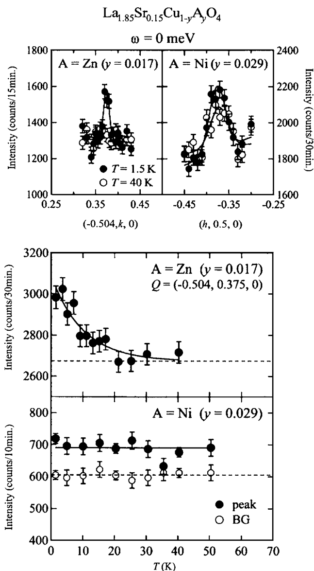
FIG. 12. The incommensurate elastic peak intensities as a function of temperature for \text{La}_{1.85}\text{Sr}_{0.15}\text{Cu}_{1-y}\text{Zn}_y\text{O}_4 (Zn: y=0.017 ) and \text{La}_{1.85}\text{Sr}_{0.15}\text{Cu}_{1-y}\text{Ni}_y\text{O}_4 (Ni: y=0.029 ). The top figures show q profiles along (a) the k direction (trajectory C in Fig. 2) for the Zn-doped sample and (b) the h direction (trajectory D in Fig. 2) for the Ni-doped sample at 1.5 and 40 K. Solid lines represent the result of fits by a Gaussian function. (c) Temperature dependence of intensity at the peak position Q=(-0.504, 0.375, 0) for the Zn-doped sample. Solid and dashed lines are guides to the eye and estimated backgrounds. (d) Temperature dependence of peak (solid circles) and background (open circles) intensities for the Ni-doped sample. Peak intensity corresponds to the average of intensity at Q=(-0.37, 0.5, 0) , (-0.38, 0.5, 0) , and (-0.39, 0.5, 0) , and background intensity corresponds to the average of intensity at Q=(-0.32, 0.5, 0) and (-0.44, 0.5, 0) . Solid and dashed lines are guides to the eye of peak and background.
