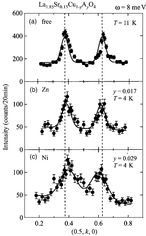
FIG. 10. Q profiles along the k direction (trajectory B in Fig. 2) for (a) \text{La}_{1.85}\text{Sr}_{0.15}\text{CuO}_4 , (b) \text{La}_{1.85}\text{Sr}_{0.15}\text{Cu}_{1-y}\text{Zn}_y\text{O}_4 (Zn: y=0.017 ), and (c) \text{La}_{1.85}\text{Sr}_{0.15}\text{Cu}_{1-y}\text{Ni}_y\text{O}_4 (Ni: y=0.029 ) at \omega=8 meV under the high-resolution condition. These data were taken at low temperature. Solid lines are the result of fits with assuming two equivalent Gaussian peaks at (0.5, 0.5 \pm \delta, 0) . Vertical dashed lines denote peak positions for (a) \text{La}_{1.85}\text{Sr}_{0.15}\text{CuO}_4 estimated by fitting.
