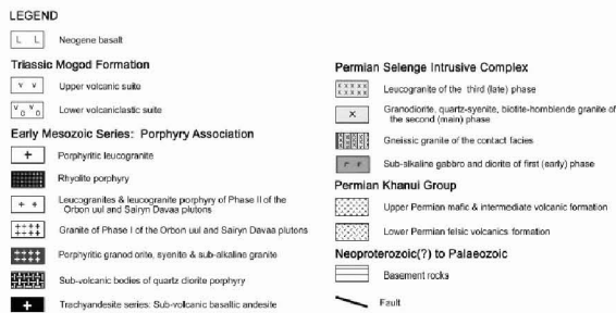
FIGURE 1. Geological map of the Erdenet area (Koval et al., 1985).
