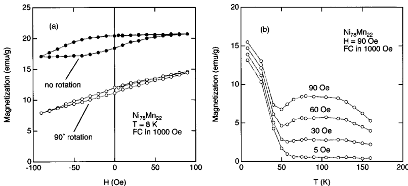
FIG. 3. (a) The magnetization of the plate sample of \text{Ni}_{78}\text{Mn}_{22} is measured as a function of applied field, where the sample was rotated 90° in a zero field after cooling of the sample to the measuring temperature in a field of 1 kOe. In addition, the magnetization curve under the FC condition with H_{\text{cool}} of 1 kOe, measured in a conventional way, is compared with the 90°-rotation data. (b) The FC magnetization, measured under the condition of 90° rotation, is plotted as a function of temperature.
