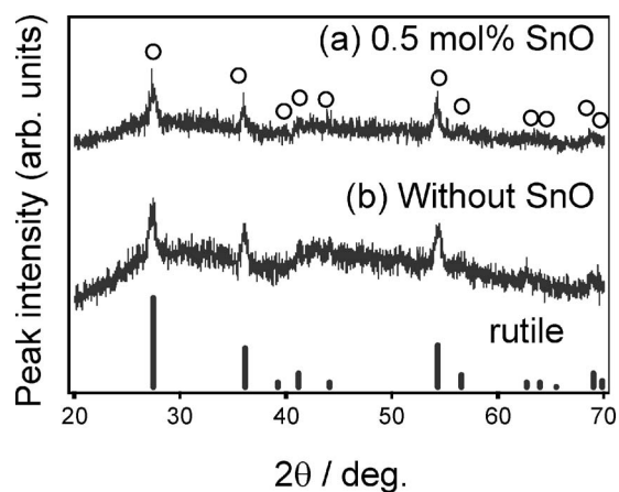
FIG. 2. XRD patterns of CaBBAT glasses with 0.5 mol % SnO (a) and without SnO (b) together with rutile (TiO 2 , Ref. 11). The \circ marks are assigned to the diffraction peaks of rutile. The glasses were heat treated for 3 h at 630 °C.
