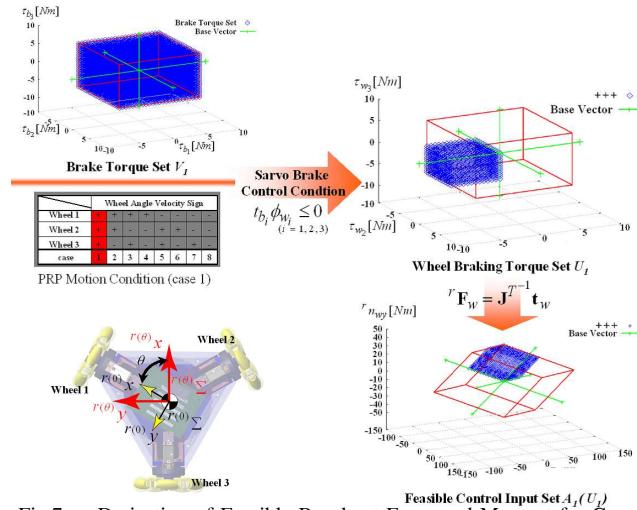
Fig.7 . Derivation of Feasible Resultant Force and Moment for Control
