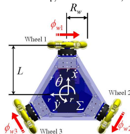
Fig.4 . Configuration and Robot Coordinates of PRP (Top View)
