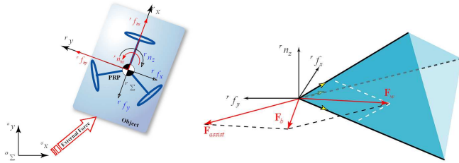
Fig.8 . (a)PRP with External Force and Moment during Object Transportation, (b)Relationship of {}^rF_{assist} , {}^rF_b and {}^rF_w
