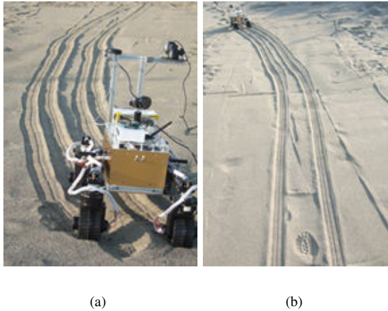
Fig. 7. Tracks produced by the wheels of the rover at the end of the traverse of a sandy slope: (a) front view, (b) rear view
