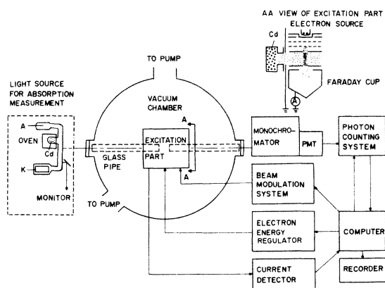
FIG. 2. Block diagram of the experimental apparatus. He-Cd tube and the two glass pipes drawn by broken lines were inserted into the position shown in the figure, only for measuring the Cd-atom density with the absorption method.
