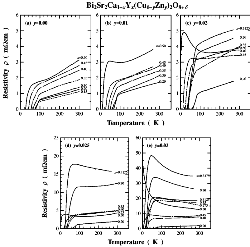
FIG. 1. Temperature dependence of the electrical resistivity \rho for \text{Bi}_2\text{Sr}_2\text{Ca}_{1-x}\text{Y}_x(\text{Cu}_{1-y}\text{Zn}_y)_2\text{O}_{8+\delta} . (a) y=0.00 , (b) y=0.01 , (c) y=0.02 , (d) y=0.025 , (e) y=0.03 .
