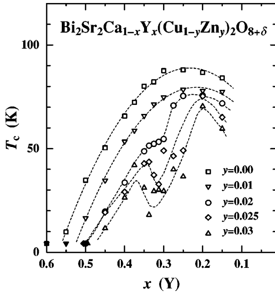
FIG. 2. Y-concentration x dependence of T_c , defined as the midpoint of the superconducting transition curve in the \rho vs T plot, for \text{Bi}_2\text{Sr}_2\text{Ca}_{1-x}\text{Y}_x(\text{Cu}_{1-y}\text{Zn}_y)_2\text{O}_{8+\delta} . Closed symbols indicate samples which are not superconducting above 4.2 K. Dashed lines are guides to the eye.
