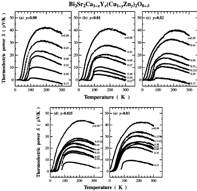
FIG. 3. Temperature dependence of the thermoelectric power S for \text{Bi}_2\text{Sr}_2\text{Ca}_{1-x}\text{Y}_x(\text{Cu}_{1-y}\text{Zn}_y)_2\text{O}_{8+\delta} . (a) y=0.00 , (b) y=0.01 , (c) y=0.02 , (d) y=0.025 , (e) y=0.03 .
