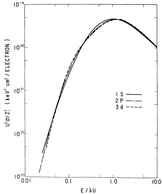
FIG. 3. Scaled ionization cross sections for the 1s (solid curve), 2p (dash-dot curve), and 3d (dashed curve) electrons calculated from the BEA. The maximum cross section for the 1s electrons is obtained at E/\lambda U = 1.0 , while those for the 2p and 3d electrons are at E/\lambda U \approx 1.2 .
