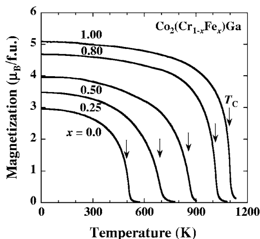
FIG. 5. Temperature dependence of the magnetization measured in a magnetic field of 0.5 T for the L2_1 -type \text{Co}_2(\text{Cr}_{1-x}\text{Fe}_x)\text{Ga} alloys. The arrows indicate the Curie temperature T_C .
