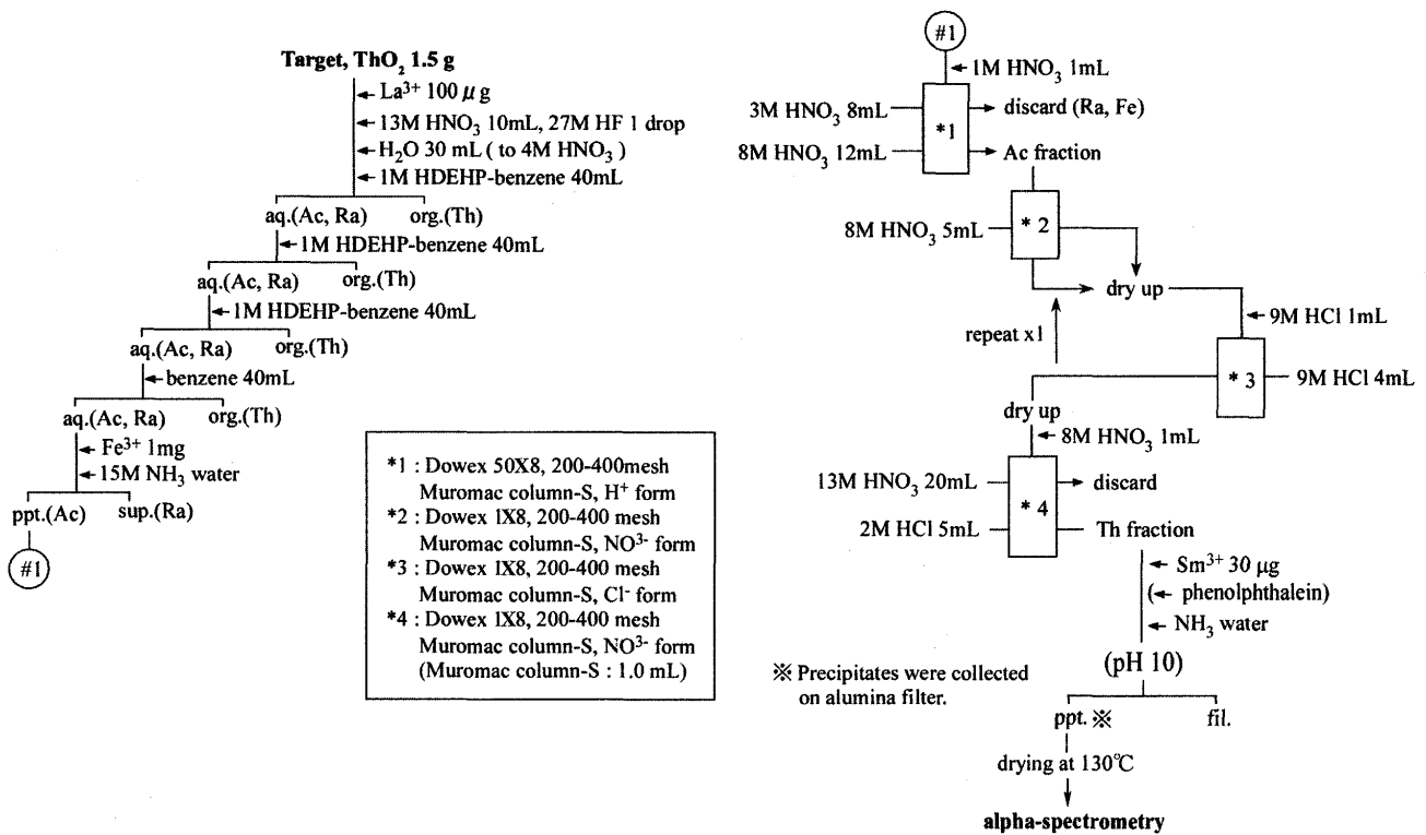
Fig.1. Chemical procedure for preparation of the 229m,g Th sample.
