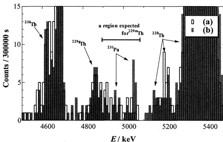
Fig.3. Expanded \alpha -ray spectra acquired over a counting duration of 3 \times 10^5 s, starting 10 minutes after the chemical separation (a), and acquired 1 week after the chemical separation (b).
