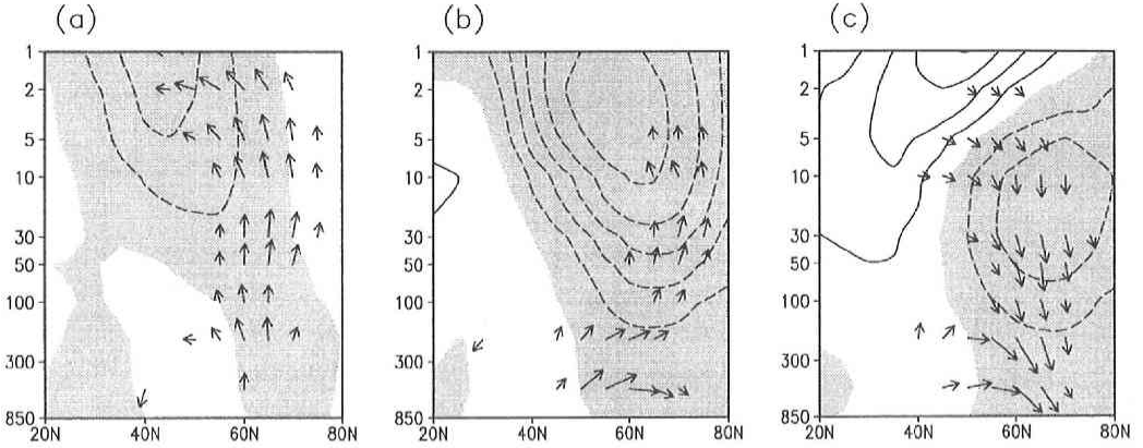
Fig. 1. Heterogeneous regression map of the leading E-SVD between the zonal-mean zonal wind (contour) and (the vertical component of) the E-P flux (vector). Meridional component of the E-P flux is constructed by the regression. Panels a, b and c correspond to the first, second and third months, respectively. The contour is 2 m/sec and the dashed lines indicate negative values. Zero contour line is omitted and negative values are shaded. The E-P flux is scaled by the reciprocal square root of pressure.
