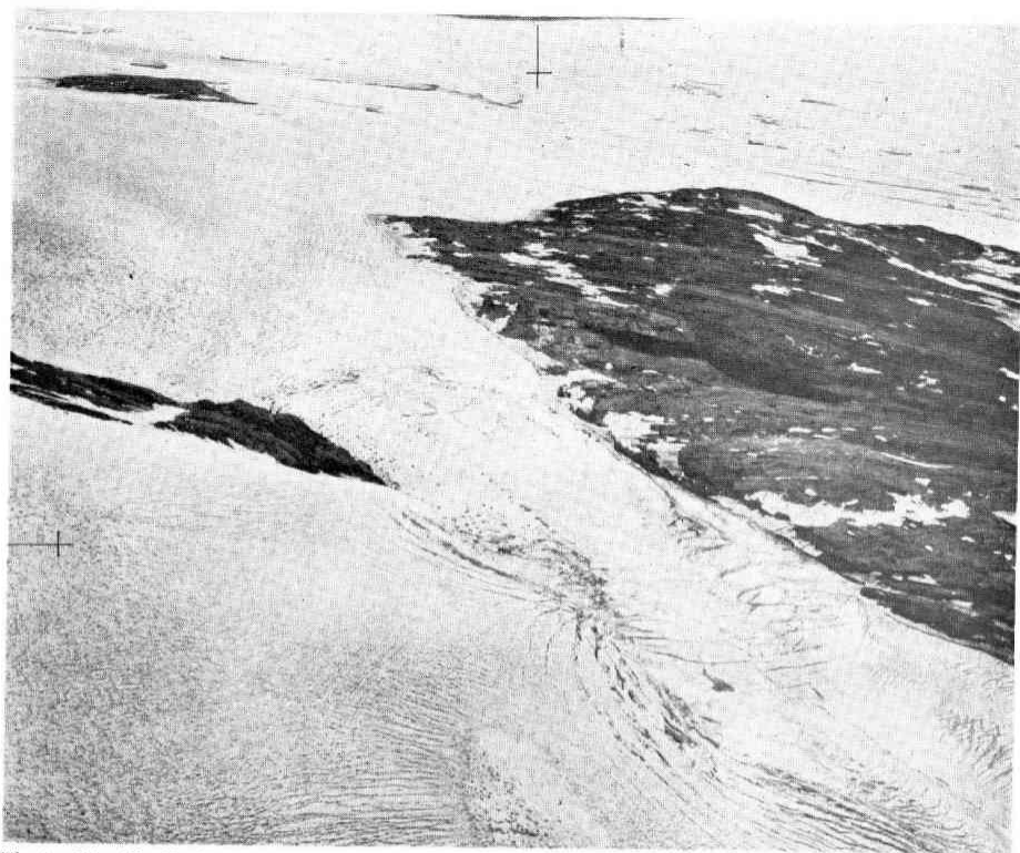
Photo 26 Skallevikhalsen Glacier. Ice free areas are Skallevikhalsen (left), Skallen (right) and Hjartöy Island (upper left)*.
