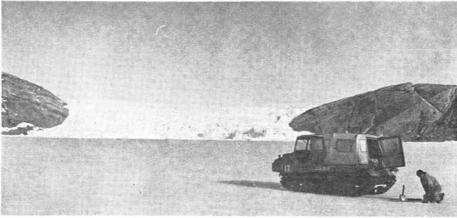
Photo 13 Ice fall of Hamna Glacier.
