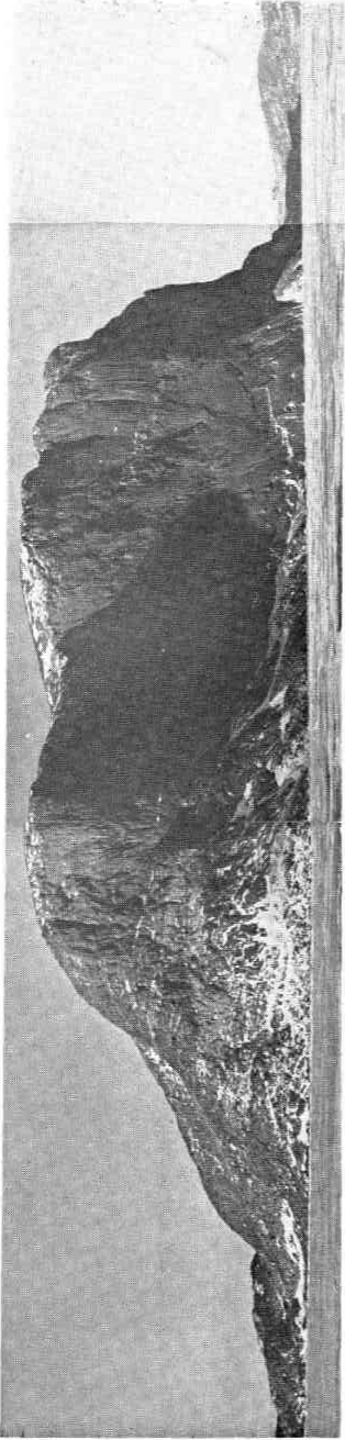
Photo 19 Northern fjord wall of Skjegget and Langpollen (Bay). The southern fjord wall has lost.
