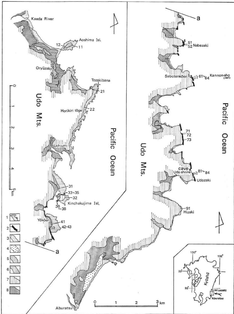
Fig. 1 Geomorphological map
