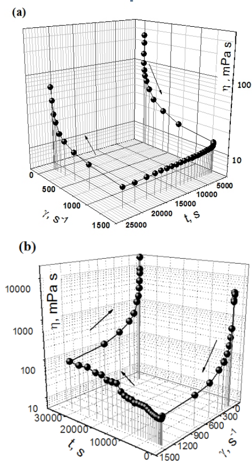
Figure 8. The dependence of viscosity on shear rate in time for 9 wt.% (b) and 13 wt.% (a) silica dispersion in solution of 0.1 M LiCl
