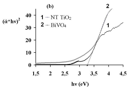
Figure 9. The optical spectral characteristics films TiO 2 -1 and TiO 2 (with thickness 500 nm)/ BiVO 4 (with thickness 2 μm) – 2 where: (a) light absorption spectra (b) light absorption spectra in coordinates (α* hν ) 2 from hν .
