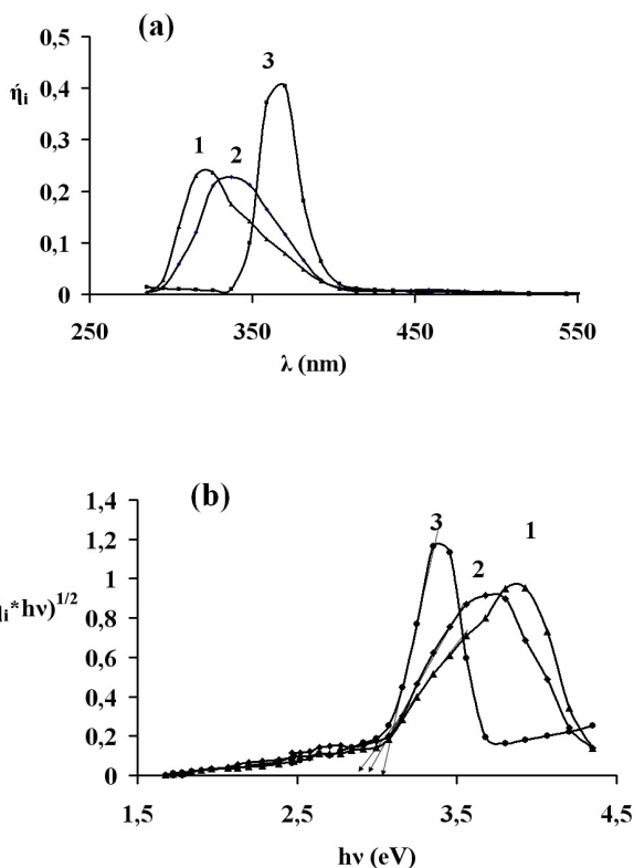
Figure 6. The photocurrent quantum yield spectra in the coordinates \eta(\lambda) (a) and (\eta \cdot hv)^{1/2}(hv) (b): 1– TiO 2 , 2– TiO 2 /V 2 O 5 , 3 – co-deposited TiO 2 /V 2 O 5 (anodic deposition at potential 1.5V).
