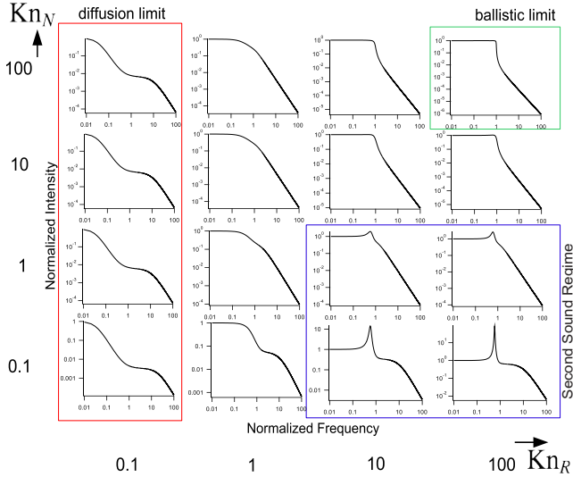
FIG. 5. (Color online) A chart of light-scattering spectra from a phonon gas for combinations of (Kn_R, Kn_N) . All the spectra are plotted on log-log scales. We set n_{max}=5 and \gamma_6=\gamma_\infty in calculating these spectra.
