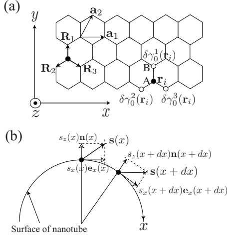
FIG. 3. (a) A hexagonal unit cell of graphene consists of A (closed circle) and B (open circle) atoms. \mathbf{a}_1 and \mathbf{a}_2 are lattice vectors. \mathbf{R}_a ( a=1,2,3 ) are vectors pointing to the nearest-neighbor B sites from an A site. For the coordinate system of (x,y) , the \mathbf{R}_a ( a=1,2,3 ) are written, respectively, as \mathbf{R}_1=a_{cc}\mathbf{e}_y , \mathbf{R}_2=-\sqrt{3}/2 a_{cc}\mathbf{e}_x-(1/2)a_{cc}\mathbf{e}_y , and \mathbf{R}_3=(\sqrt{3}/2)a_{cc}\mathbf{e}_x-(1/2)a_{cc}\mathbf{e}_y where a_{cc} is the carbon-carbon bond length and \mathbf{e}_x ( \mathbf{e}_y ) is the dimensionless unit vector for the x axis ( y axis). Local modulations of the hopping integral are defined by \delta\gamma_0^a(\mathbf{r}_i) ( a=1,2,3 ) where \mathbf{r}_i is the position of an A atom. (b) The displacement vector for the RBM, \mathbf{s}(x) , is decomposed in terms of the normal s_z(x) and tangential s_x(x) components. The derivative of the normal unit vector \mathbf{n}(x) with respect to x gives a component along \mathbf{e}_x(x) , which modifies the net displacement along the x direction.
