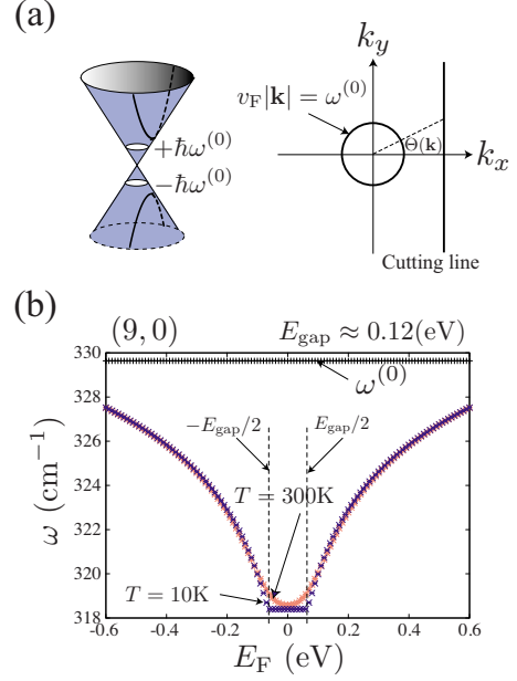
FIG. 4. (Color online) (a) The decay width is zero because of E_{\text{gap}} > \hbar\omega^{(0)} . This is shown by the relative positions of the cutting line and the equienergy contour circle satisfying v_F|\mathbf{k}| = \omega^{(0)} with respect to the Dirac point. (b) The E_F dependence of the RBM frequency in the case of the (9,0) zigzag SWNT at room temperature (red curve) and at 10 K (blue curve). We plot \omega^{(0)} as the black line for comparison.
