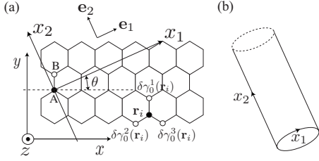
FIG. 7. (a) We define the coordinate system (x_1, x_2) for graphene. \mathbf{e}_1 ( \mathbf{e}_2 ) is the dimensionless unit vector for the x_1 axis ( x_2 axis). (b) x_1 ( x_2 ) is the coordinate around (along) a tube axis. The periodic boundary condition along the x_1 axis corresponds to a carbon nanotube with chiral angle \theta .
