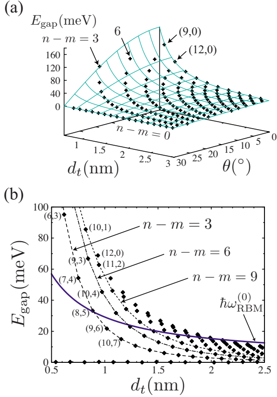
FIG. 2. (Color online) (a) The dependence of the curvature-induced energy gap E_{\text{gap}} on the chiral angle \theta and tube diameter d_t . The surface is a plot of Eq. (3) which reproduces well the calculated results. (b) The d_t dependence of E_{\text{gap}} , which is given as a one-dimensional projection of (a) onto the d_t axis. We plot the energy of the RBM, \hbar\omega^{(0)} of Eq. (1), as a solid blue curve for comparison. The points on the dashed, dot-dashed, and dotted curves satisfy n-m=3, 6, 9 , respectively.
