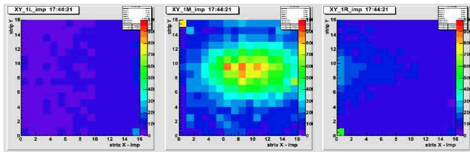
FIGURE 1. Implantation pattern on DSSSD for ^{213}\text{Fr} settings during 4 second spill time.
