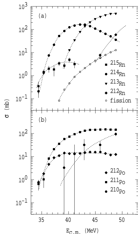
FIG. 1. (a) The measured cross sections for fission and the production of Rn isotopes, and (b) of Po isotopes following the reaction ^9\text{Be} + ^{208}\text{Pb} . The dashed lines guide the eye.
