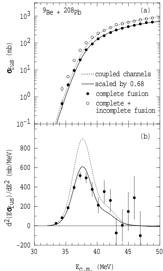
FIG. 2. (a) The excitation function for complete fusion (filled circles) and (b) the barrier distribution for the reaction {}^9\text{Be} + {}^{208}\text{Pb} . The dashed line is the result of a coupled channels calculation (see text) which ignores breakup effects. The full line is the same calculation scaled by 0.68. The sum of measured complete and incomplete fusion cross sections is given by the hollow circles.
