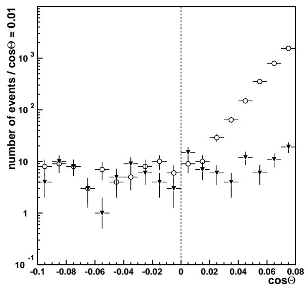
FIG. 1. Zenith-angle distribution of throughgoing muons near the horizon observed by Super-K. Filled triangles (open circles) indicate events coming from the 180^\circ azimuthal region where the rock overburden is thick (shallow). Most of the downwardgoing ( \cos \Theta > 0 ) muons denoted by filled triangles are induced by atmospheric neutrinos.
