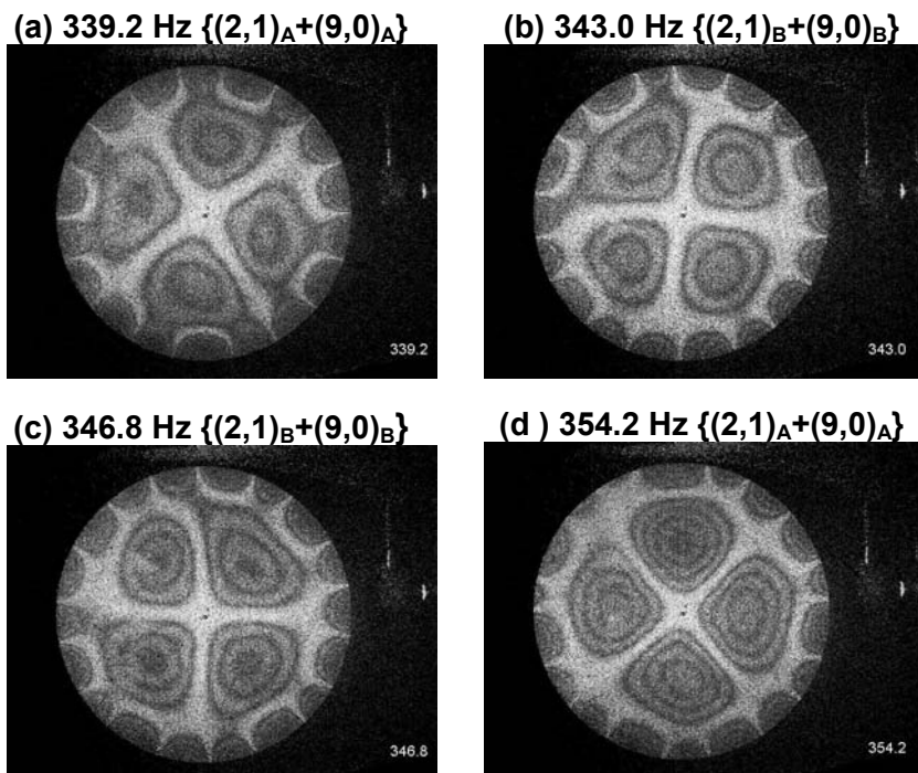
Figure 8: [(9,0) + (2,1)] mixed modes
