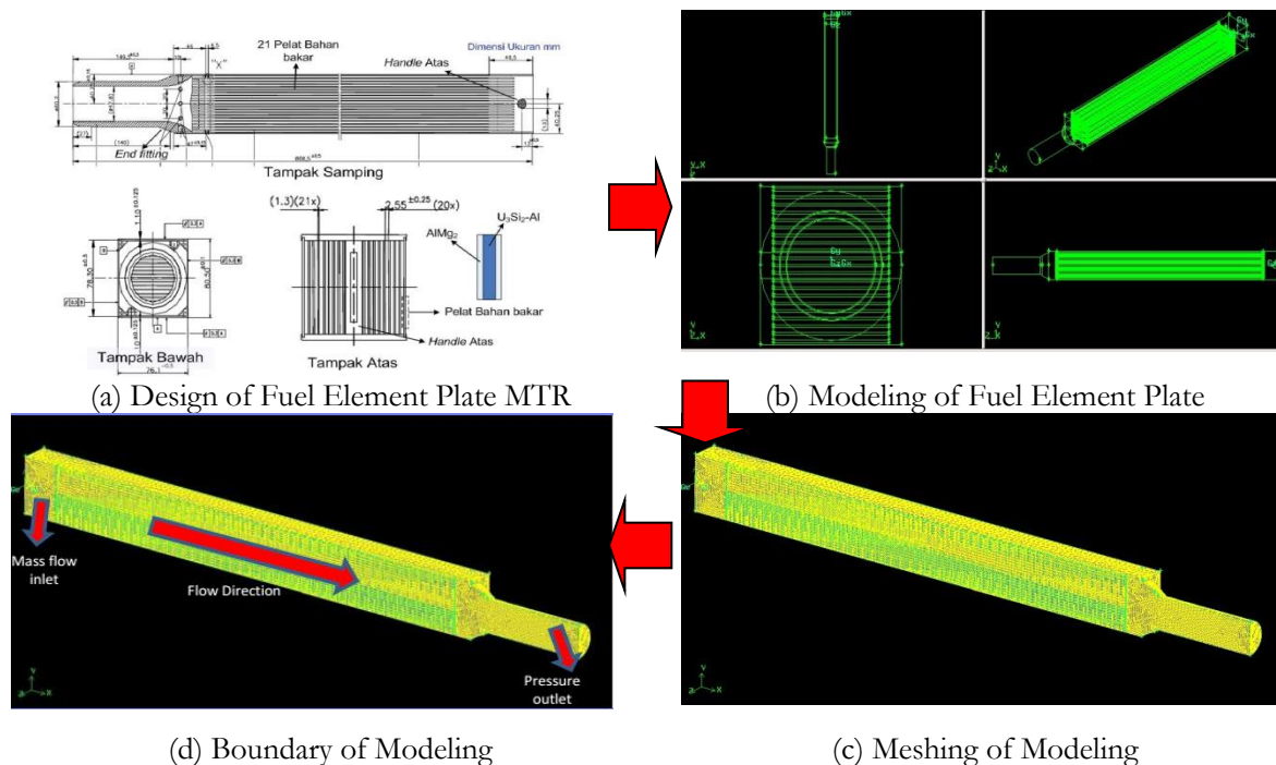
Fig. 2. Modeling of fuel element plate MTR.
