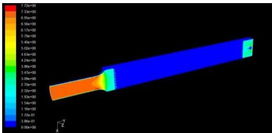
Fig. 7. Distribution of velocity flow of fuel element MTR use non porous media.
