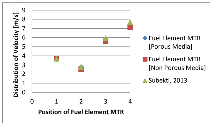
Fig. 10. Comparison of the velocity distribution.
