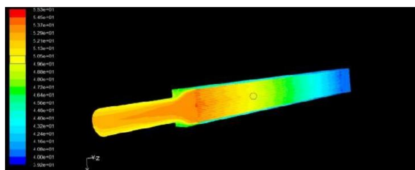
Fig. 3. Distribution of temperature for fuel element MTR use non porous media.
