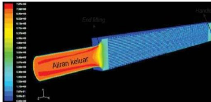
Fig. 9. Distribution of velocity flow of fuel element MTR [10].
