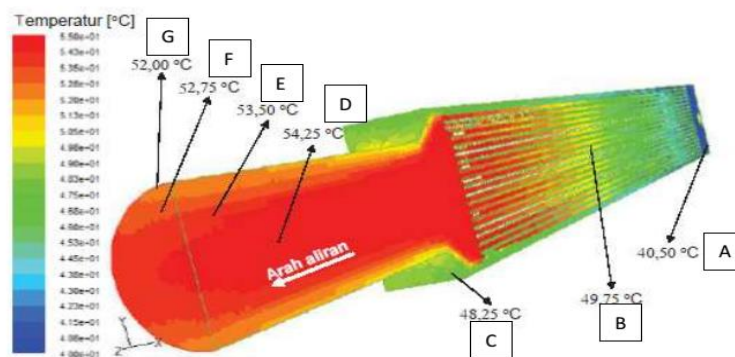
Fig. 5. Distribution of temperature for fuel element MTR [10].
