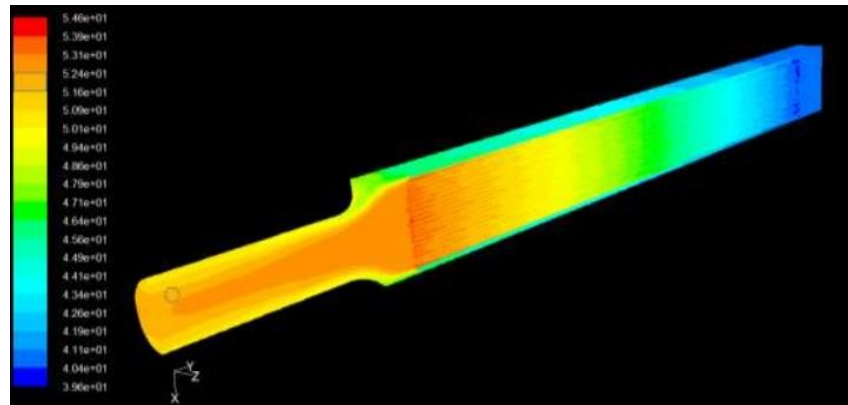
Fig. 4. Distribution of temperature for fuel element MTR use porous media.
