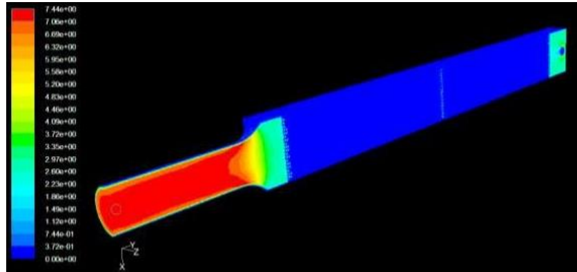
Fig. 8. Distribution of velocity flow of fuel element MTR use porous media.
