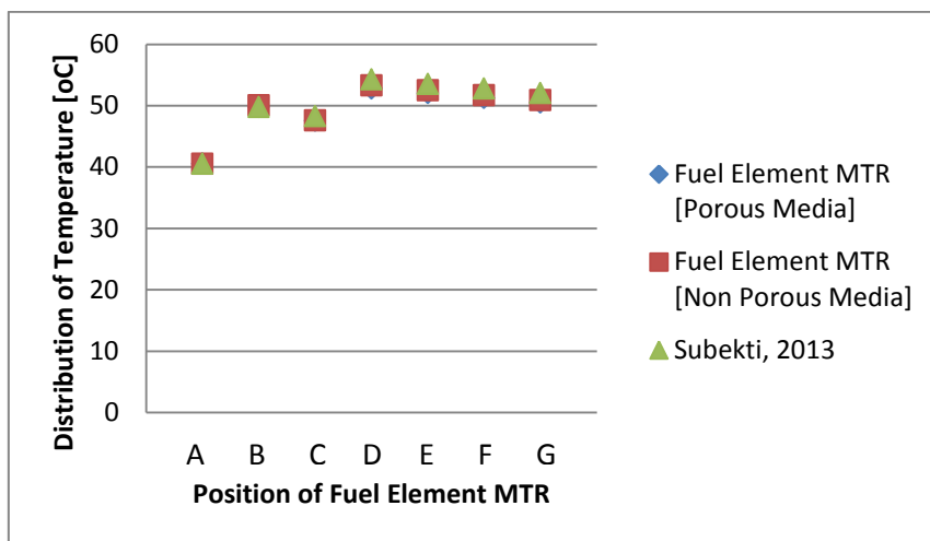
Fig. 6. Comparison of temperature distribution between researched by Subekti (2013) [10].
