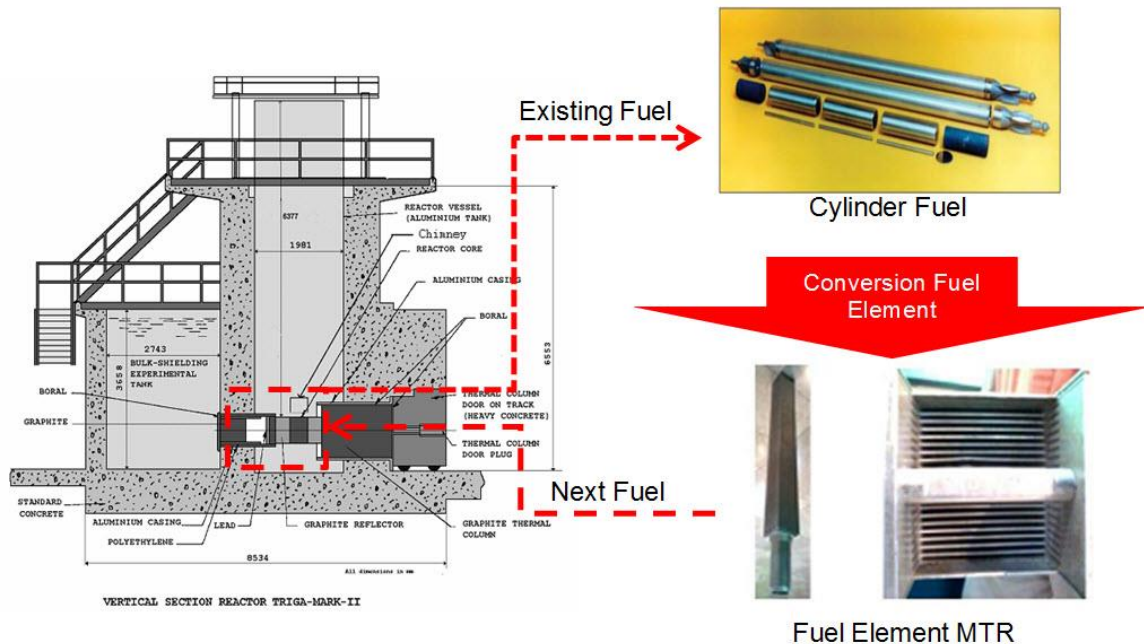
Fig. 1. Modification of Research Reactor TRIGA Bandung With Fuel Element Plat MTR.
