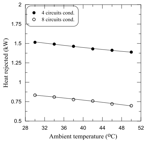
Fig. 8. Heat rejected from two phase region versus ambient temperature for four and eight circuits' condensers.
