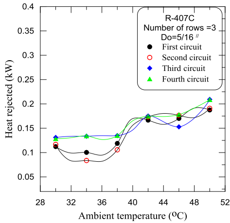
Fig. 10. Heat rejected from liquid refrigerant in each circuit of the four circuits condenser versus ambient temperature.
