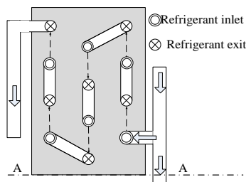
Fig. 2a. Section in four Circuits condenser showing one circuit
