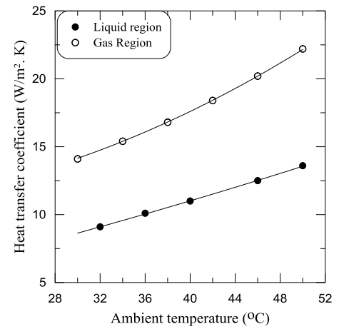
Fig. 9. Heat transfer coefficient of liquid and gas regions versus ambient temperature for four circuits' condenser.
