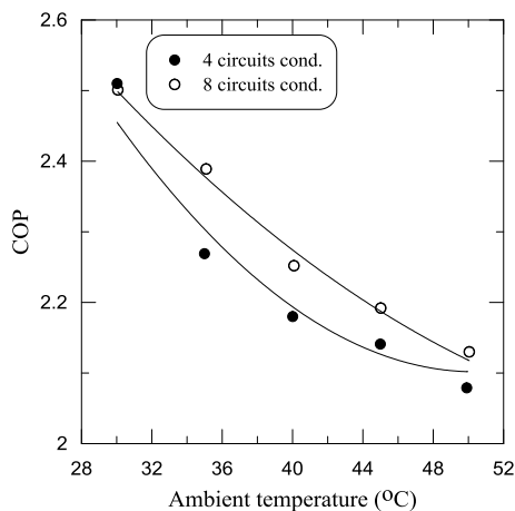
Fig. 14. Vapour compression cycle COP for the four and eight circuits condenser versus ambient temperature.
