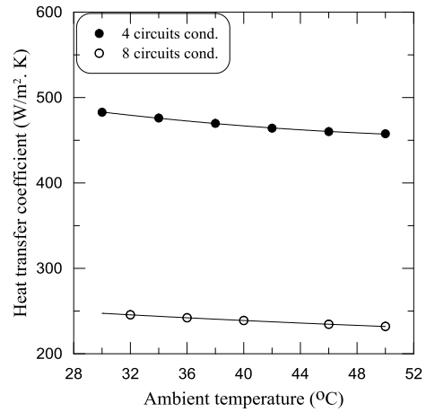
Fig. 7. Heat transfer coefficient of two phase region vs. ambient temperature for four and eight circuits condenser.
