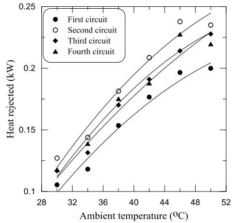
Fig. 11. Heat rejected from gas refrigerant in each circuit consist the four circuits condenser versus ambient temperature.
