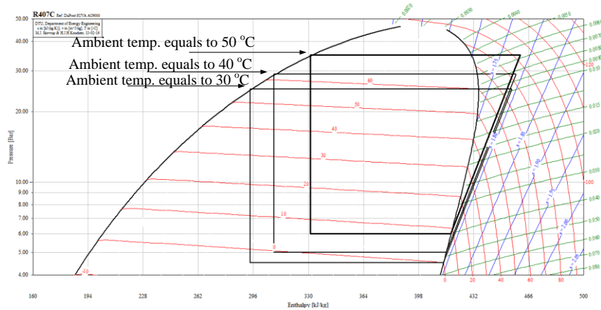
Fig. 3. Pressure-enthalpy diagram of R407C shows different refrigeration cycle operate at different ambient temperature.
