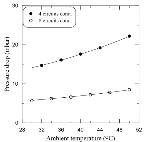
Fig. 5. Pressure drop in gas region vs. ambient temperature for both four and eight circuits' condenser.
