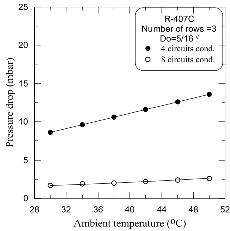
Fig. 6. Pressure drop in liquid region vs. ambient temperature for both four and eight circuits condenser.
