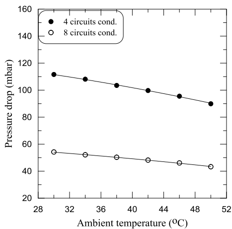
Fig. 4. Pressure drop in two phase region vs. ambient temperature for both four and eight circuits' condenser.
