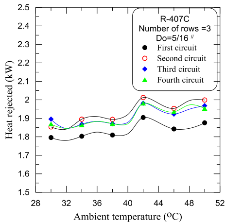
Fig. 12. Overall heat rejected from refrigerant in each circuit consist the four circuits condenser versus ambient temperature.
