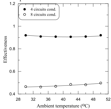
Fig. 13. Effect of ambient temperature on the effectiveness of the four and eight circuits' condenser.
