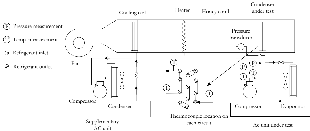
Fig. 1. Experimental rig layout.
