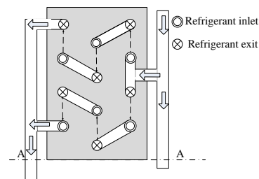
Fig. 2b. Section in eight circuit' condenser showing two circuits
