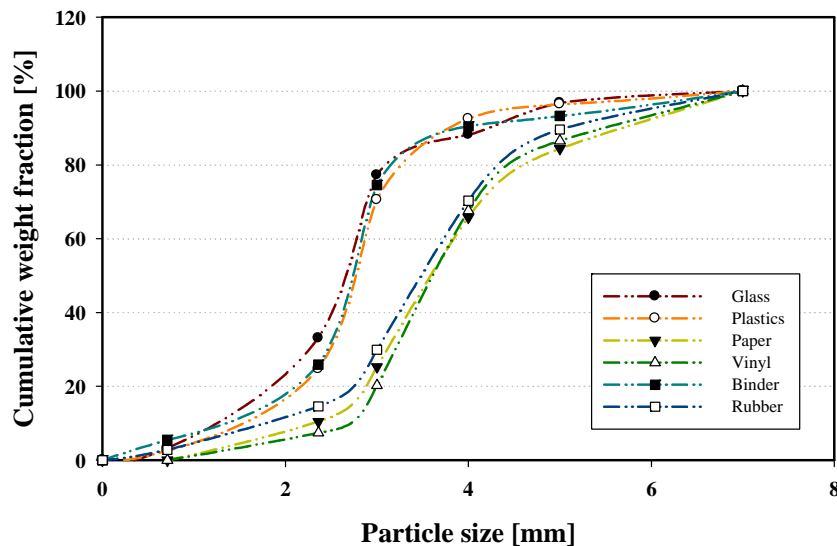
Fig. 2. Particle size distribution of the components of CFL with cumulative weight fraction.
