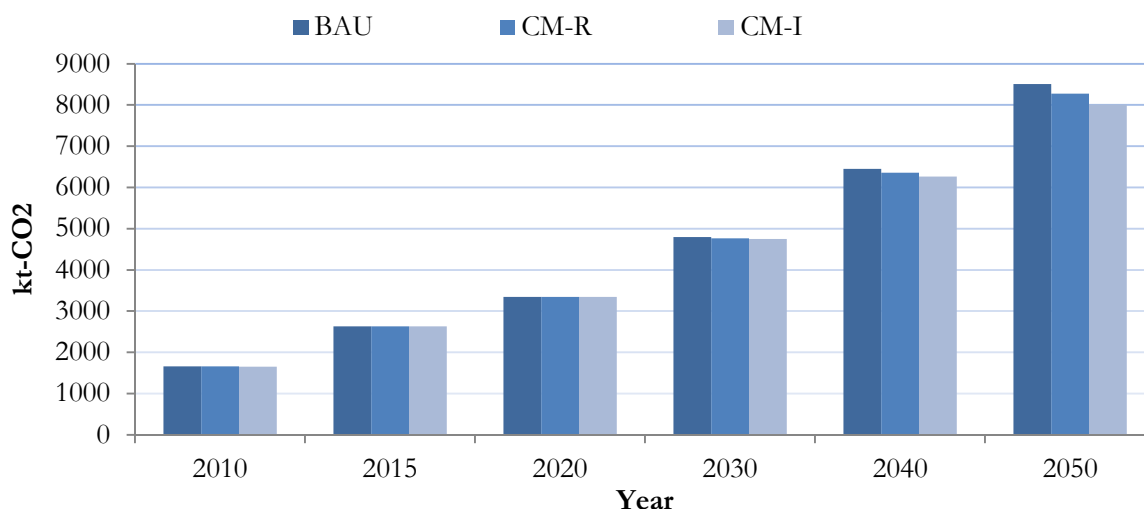
Fig. 7. Comparison of CO 2 emissions in the BAU, CM-R and CM-I scenarios.
