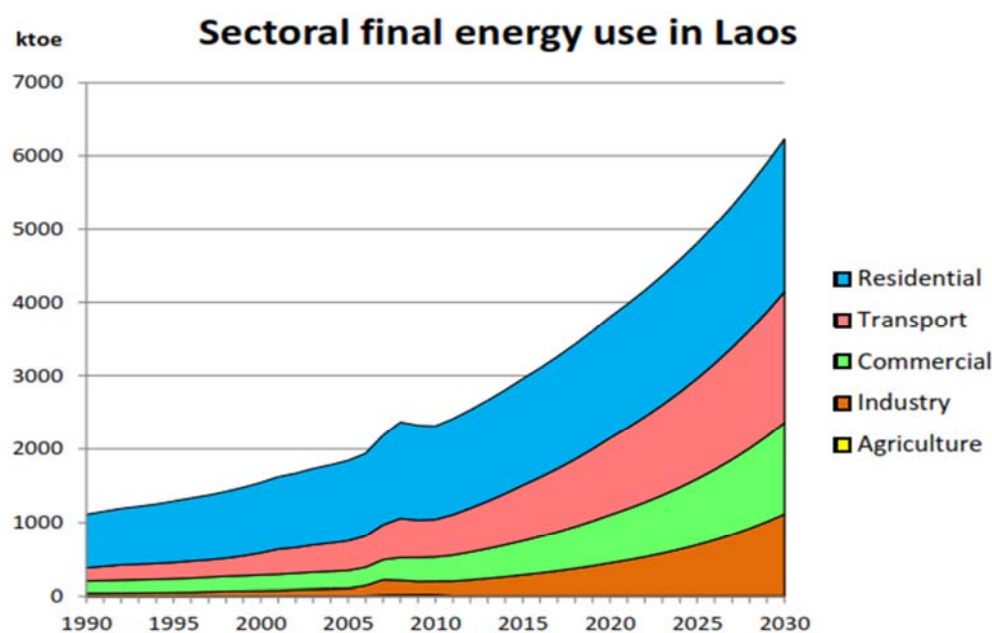
Fig. 1. Statistical record and projection of Lao final energy consumption in the BAU [4].
