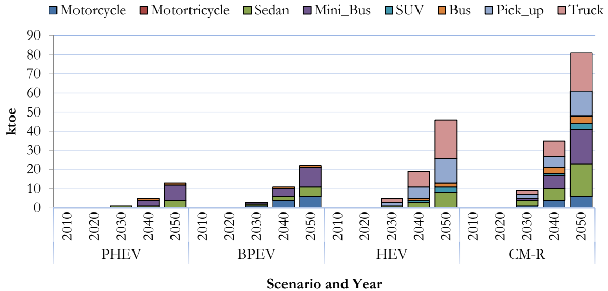
Fig. 5. Reduction in fossil fuel by mitigation actions in the realistic scenario.
