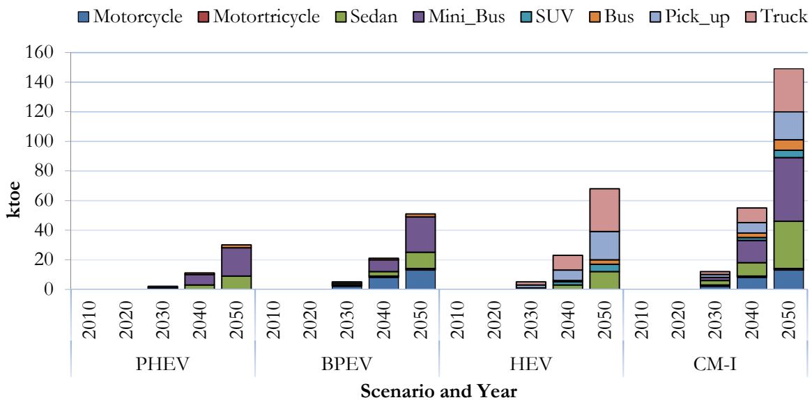
Fig. 6. Reduction in fossil fuel by mitigation actions in the idealistic scenario.
