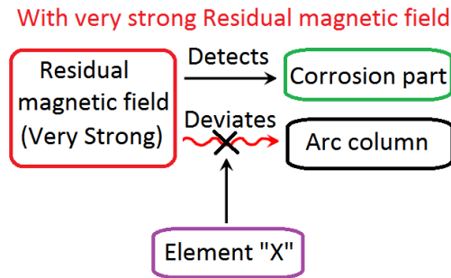
Fig. 8. Graphical models for new problem model.
