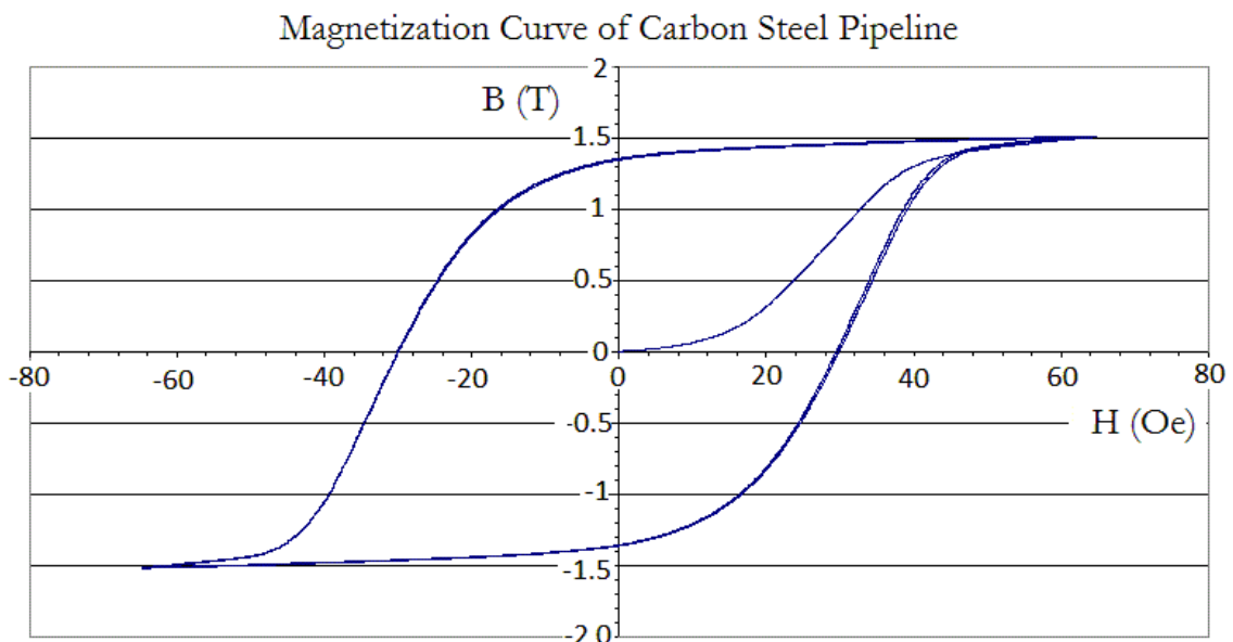
Fig. 20. Magnetic property of the carbon steel pipeline (API grades).
