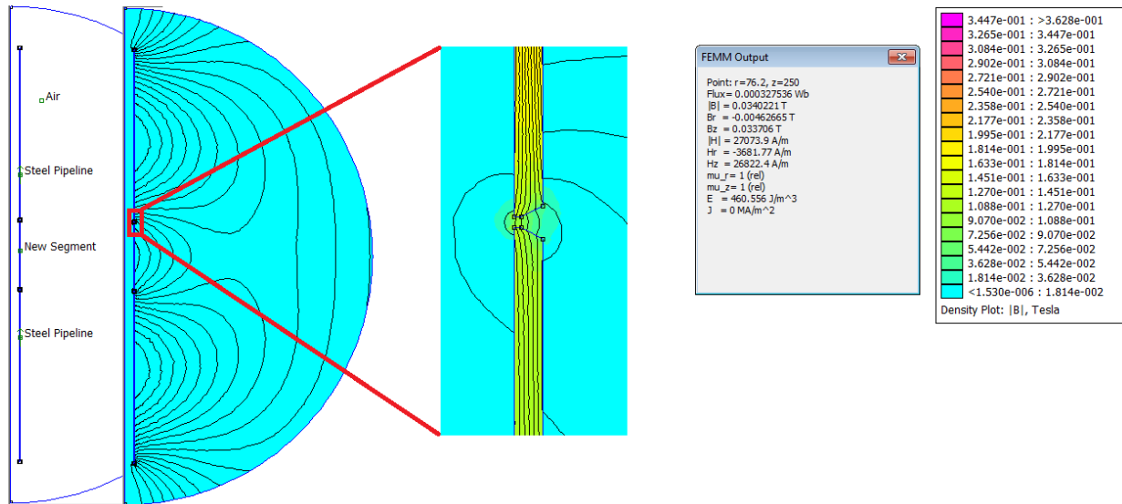
Fig. 21. Magnetic field simulation with no compensation.
