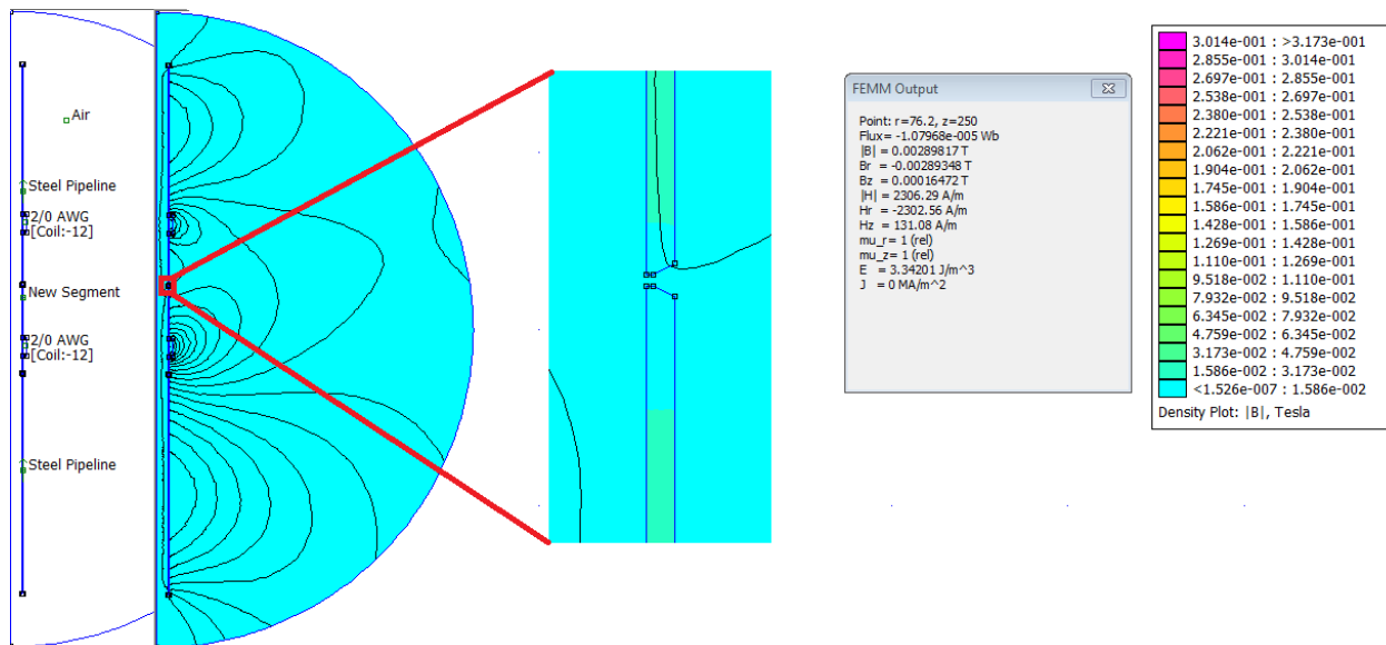
Fig. 22. Magnetic field simulation with compensation.
