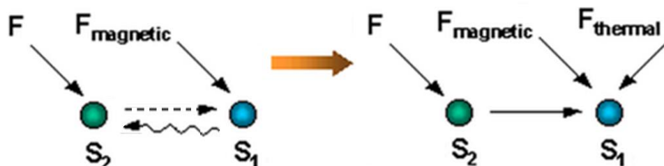
Fig. 10. Standard solution 1.2.5 “Switching Off” a magnetic influence.
