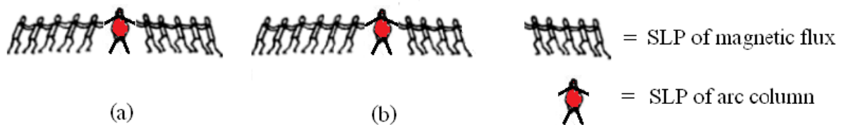
Fig. 16. Smart Little People (SLP) of components of the system in the conflict zone; (a) with no unbalance of magnetic flux around arc column; (b) with unbalance of magnetic flux around arc column.
