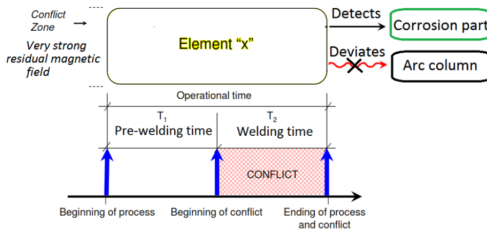
Fig. 12. Ideal Final Result (IFR-1).
