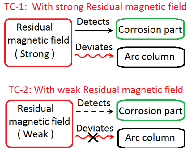
Fig. 6. Graphical models for the technical contradictions.
