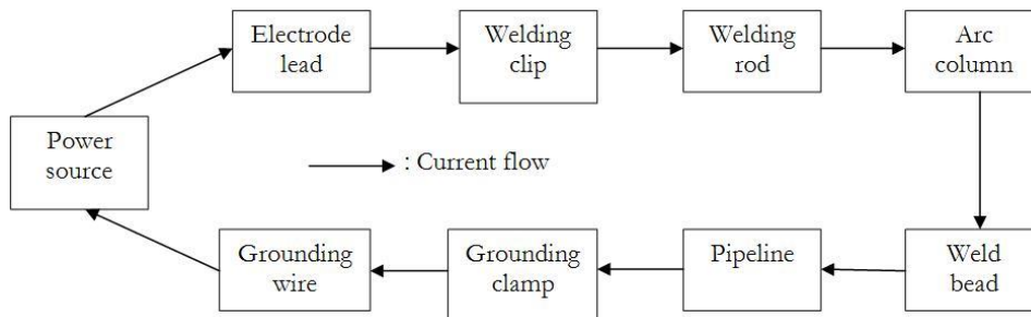
Fig. 3. Flow Analysis of current in pipeline welding system.
