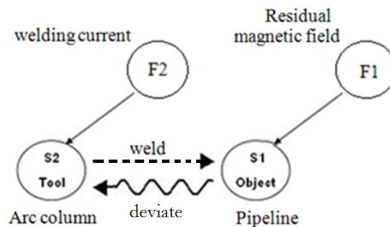
Fig. 9. Substance-field modeling and analysis.
