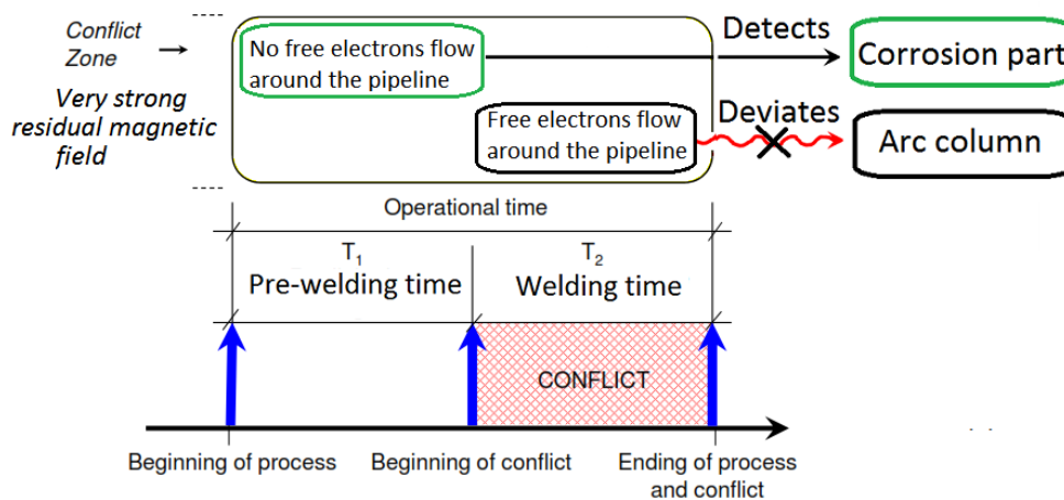
Fig. 15. Physical contradiction for the micro-level.
