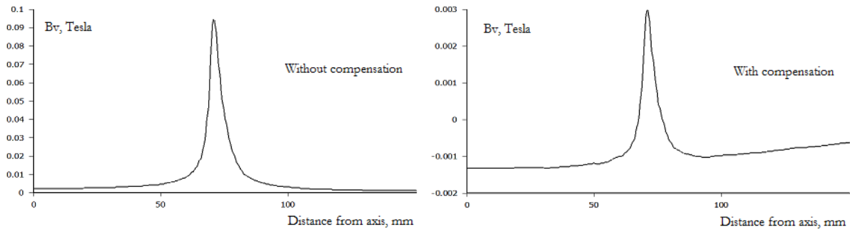
Fig. 23. Magnetic field variation at the V-groove from the axis inside the pipe to outside space.
