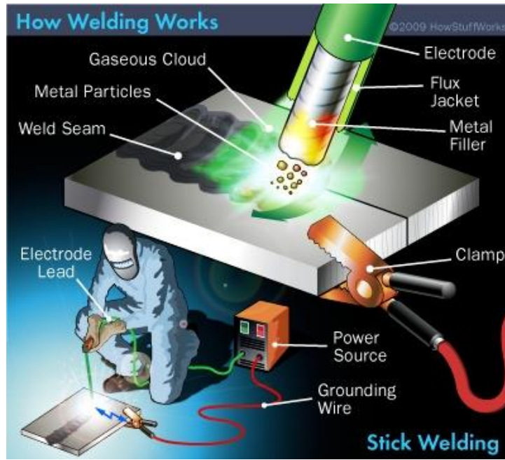
Fig. 2. The process of arc welding (HowStuffWorks [8]).
