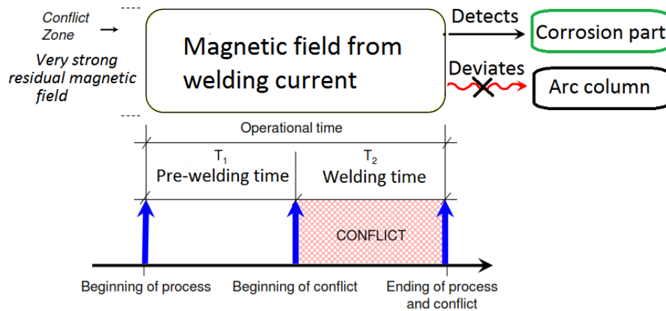
Fig. 13. Intensified formula for IFR-1.
