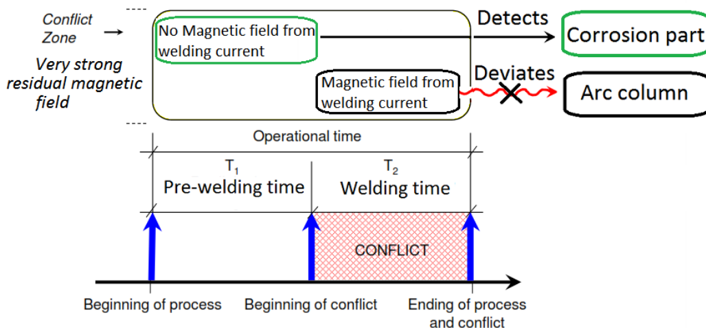
Fig. 14. Physical contradiction for the macro-level.
