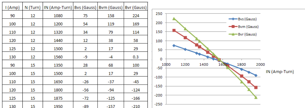
Fig. 24. The table and graphs of resultant magnetic fields at the V-groove.
