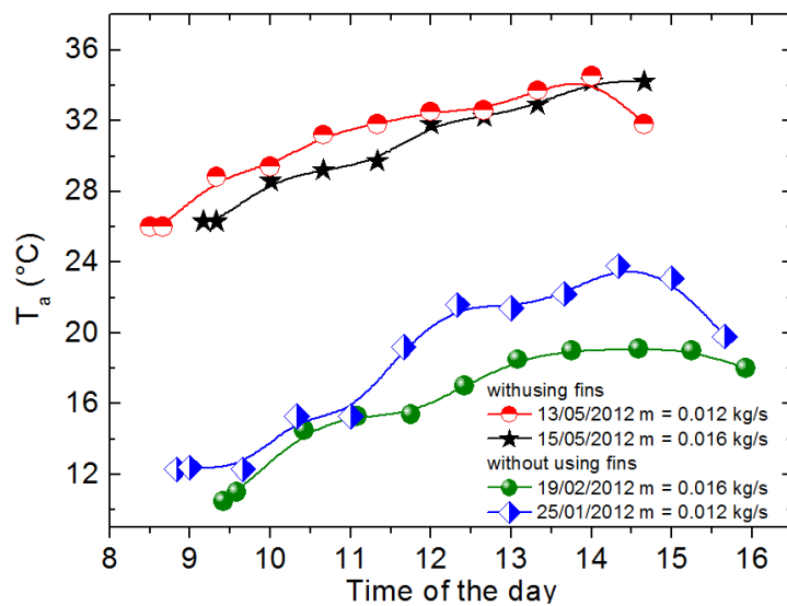
Fig. 9. Ambient temperature with and without using fins for January, February and May (2012).
