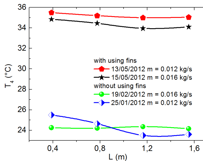
Fig. 8. Average temperature of the exterior plate with and without using fins for the months of January, February and May (2012).
