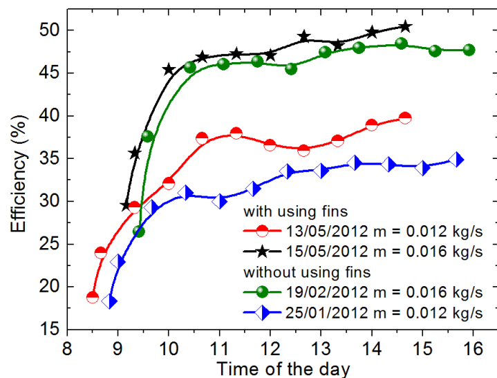
Fig. 10. Effect of the air flow on the daily efficiency of the collector, with, and without using fins for months of January, February and May (2012).
