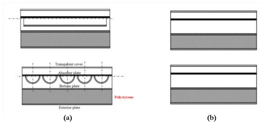
Fig. 3. Schematic views of the box solar collector.
