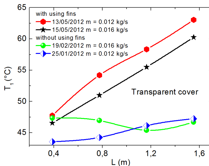
Fig. 5. Average temperature of the transparent cove with and without using fins for the months of January, February and May (2012).
