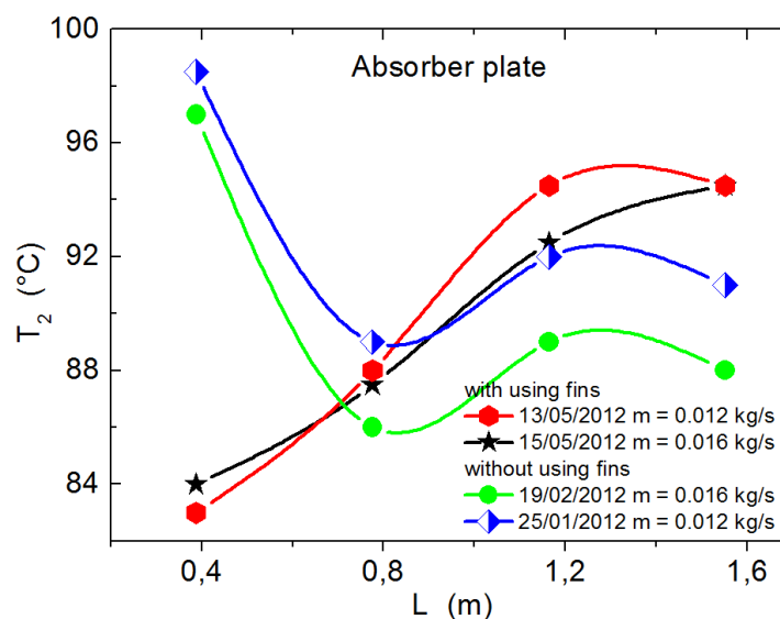
Fig. 6. Average temperature of absorber plate with and without using fins for the months of January, February and May (2012).
