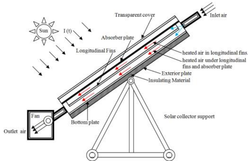
Fig. 2. Schematic views of experimental setup.
