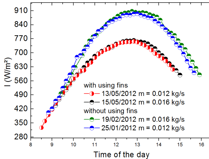
Fig. 4. Hourly variation of solar irradiation, for months of January, February and May (2012).
