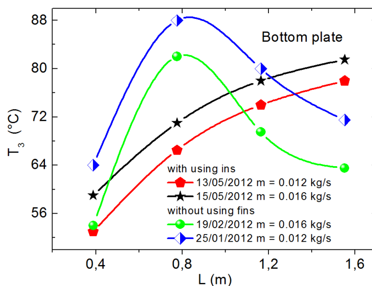
Fig. 7. Average temperature of the bottom plate with, and without using fins for months of January, February and May (2012).
