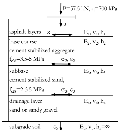
Fig. 1. Model of pavement structure (first construction stage).
