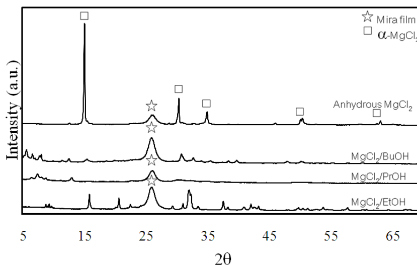
Fig. 3. XRD pattern of anhydrous MgCl 2 and porous MgCl 2 particles.
