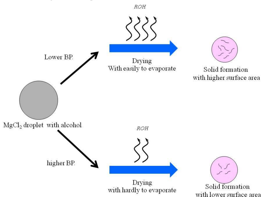
Fig. 4. Model for explanation of porosity generation in particles.
