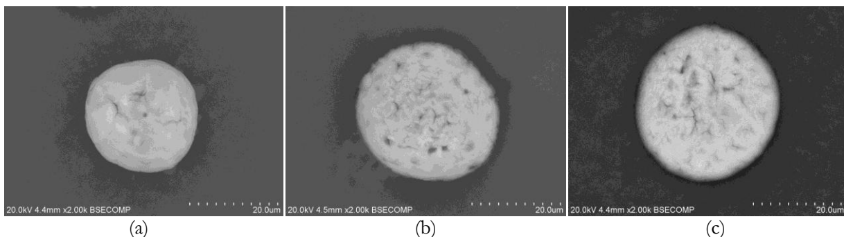
Fig. 2. Morphology of spray dried porous \text{MgCl}_2 particles with (a) ethanol, (b) n -propanol, (c) n -butanol.
