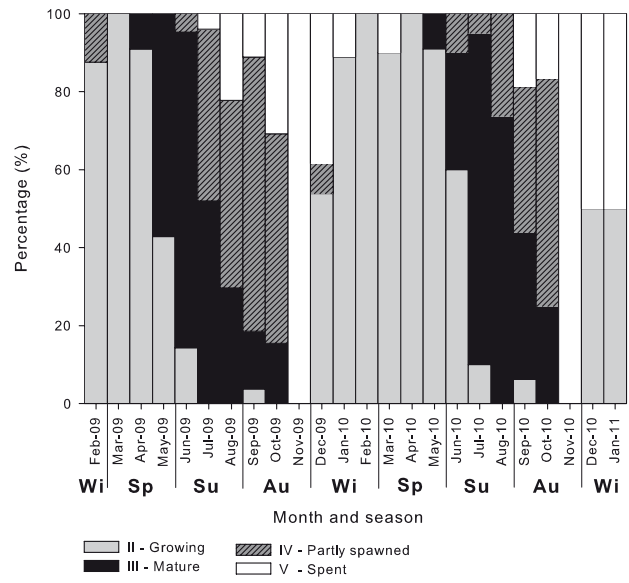
FIG. 5. – Maturity stages of H. sanctori at Gran Canaria from February 2009 to January 2011.
