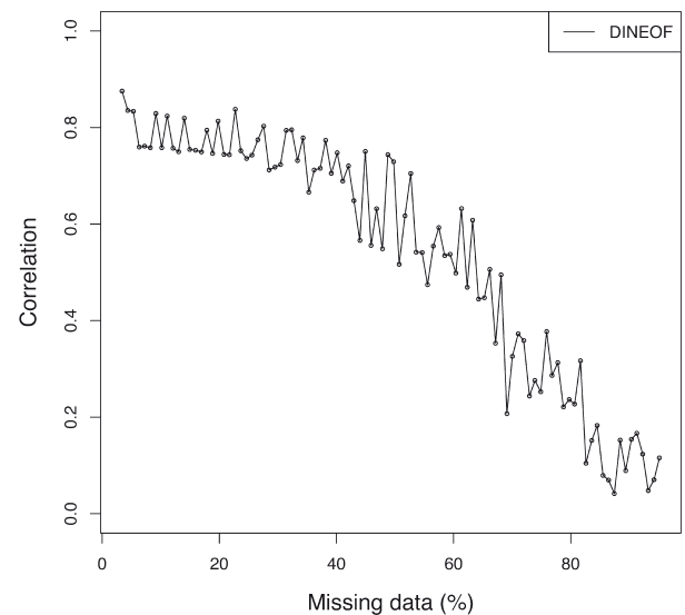
FIG. 6. – Pearson correlation between original and reconstructed data.
