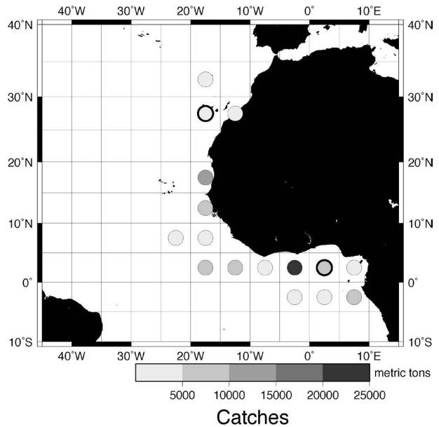
FIG. 1. – Location of the study area. The grey scale indicates the average annual catch of each area in metric tons. The two areas chosen for capture data reconstruction (Canary Islands and Gulf of Guinea) were black outlined.
