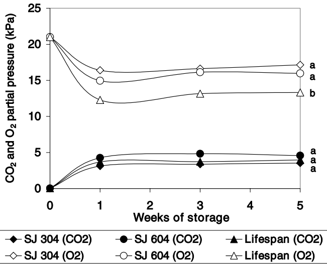
Fig. 1: Changes in partial pressures of CO 2 and O 2 inside various MAP-liners filled with 500 g sweet cherries cv. Regina, and stored at 0 °C, over a storage period of five weeks in 2003. Different letters indicate significant differences between treatments at P ≤ 0.05, Duncan's multiple range test.
