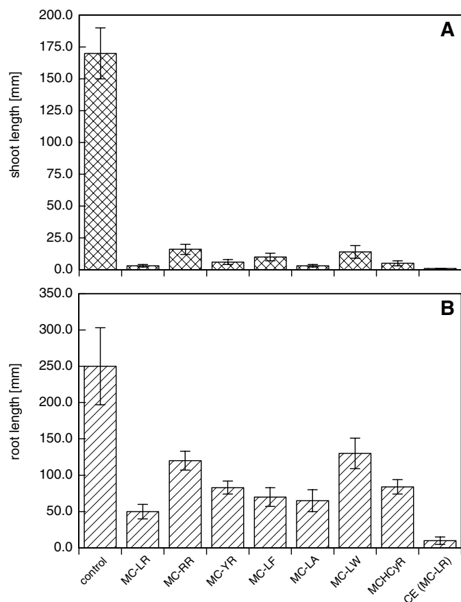
Fig. 2: Shoot length (A) and root length (B) of Z. mays seedlings after exposure to different microcystin variants.
