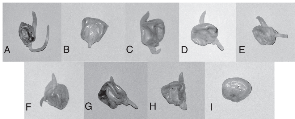
Fig. 1: Z. mays seeds exposed to different microcystin variants A) control, B) MC-LR, C) MC-RR, D) MC-YR, E) MC-LF, F) MC-LA, G) MC-LW, H) Htyr-MC, I) crude extract
