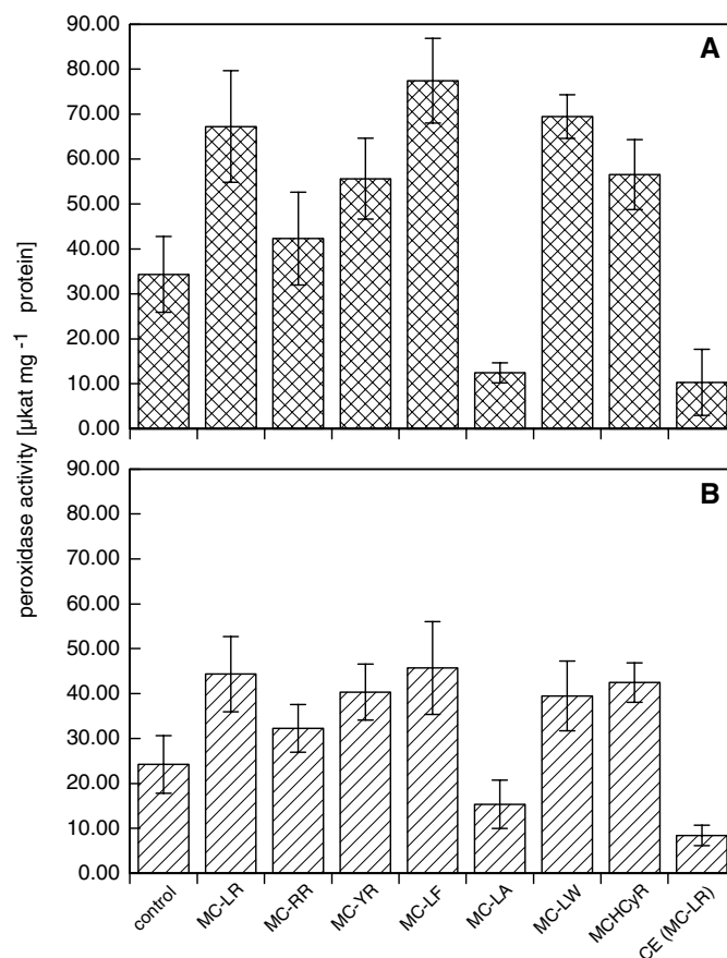
Fig. 3: Peroxidase activity in shoots (A) and roots (B) of Z. mays seedlings after exposure to different microcystin variants.
