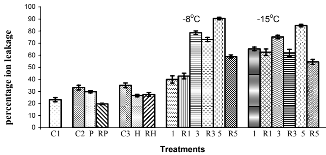
Fig. 1: Electrolyte leakage from the rootstocks of prehardened (P) at 12°C, hardened (H) at 5°C and frozen at -8°C and -15°C for 1, 3 or 5 days Miscanthus plants (-8/1, -8/3, -8/5; -15/1, -15/3 -15/5). C1 – initial control; C2 – control for prehardened plants; C3 – control for hardened and frozen plants. RP – pre-hardened plants regrowing at 20°C for 5 weeks; RH – hardened plants re-growing at 20°C for 5 weeks; R1, R2 and R3 – frozen plants at both frost temperatures for 1, 3 or 5 days respectively and regrowing at 20°C. Mean of 50 replicates \pm SE.
