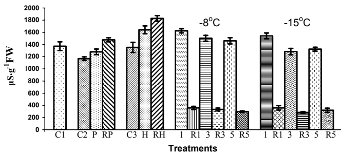
Fig. 2: Ion content [ \mu\text{S}\cdot\text{g}^{-1}\text{FW} ] in the rootstocks of prehardened, hardened and frozen Miscanthus plants. Treatment labels the same as on Fig. 1. Mean of 50 replicates \pm SE.
