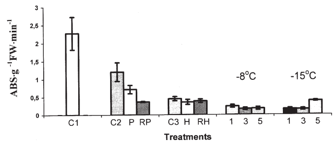
Fig. 4: Non-specific peroxidase activity in the rootstocks of prehardened, hardened and frozen Miscanthus plants. Treatment labels the same as on Fig. 1. Mean of 15 replicates \pm SE.
