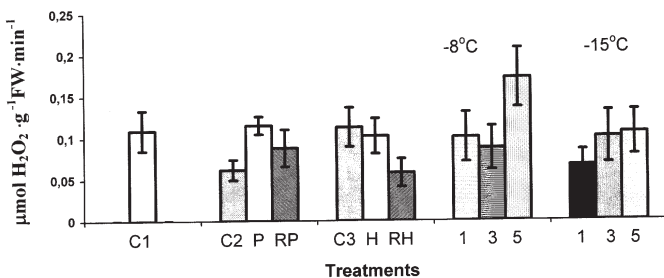
Fig. 3: Catalase activity in the rootstocks of prehardened, hardened and frozen Miscanthus plants. Treatment labels the same as on Fig. 1. Mean of 15 replicates \pm SE.
