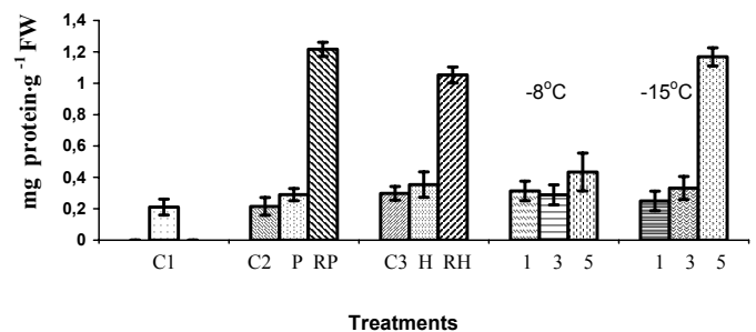
Fig. 5: Protein content in the rootstocks of prehardened, hardened and frozen Miscanthus plants. Treatment labels the same as on Fig. 1. Mean of 15 replicates \pm SE.
