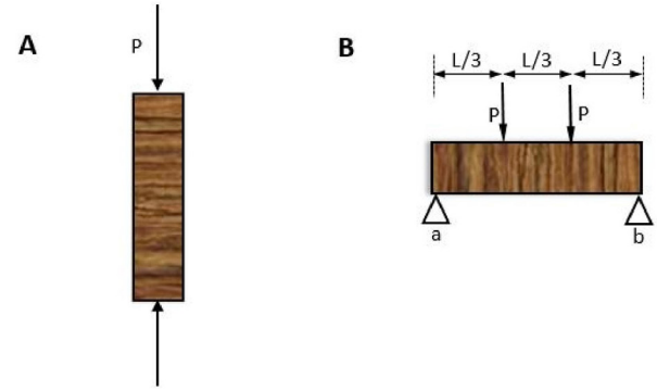
Fig. 1: A) Scheme of the compression test in trunks (P axial force applied until breakage); B) Scheme of the flexural test in branches: 'a' and 'b' were the supporting points in the extremes of the device. The P forces were applied in central third of the specimen until breakage.
