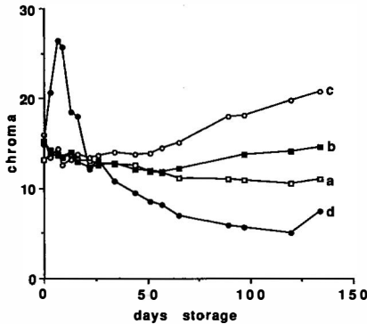
Fig. 8: Changes in chroma in models a: control, b: anthocyanins+catechin, c: anthocyanins+catechin+ferric ions, d: anthocyanins+catechin+acetaldehyde.
