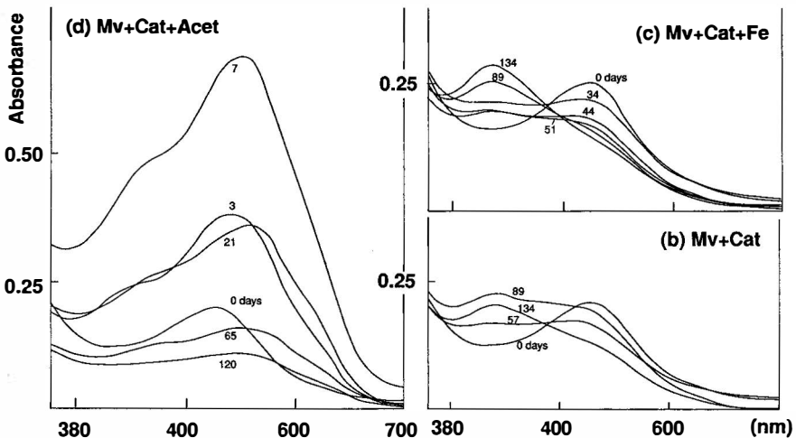
Fig. 5: Absorbance spectra changes with time for models b: anthocyanins-catechin, c: anthocyanins+catechin+ferric ions, d: anthocyanins+catechin+acetaldehyde.
