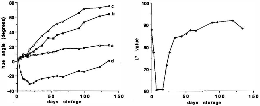
Fig. 6 (left): Changes in hue angle (degrees) in models a: control, b: anthocyanins+catechin, c: anthocyanins+catechin+ferric ions, d: anthocyanins+catechin+acetaldehyde.
