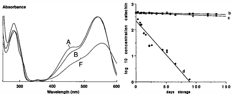
Fig. 3 (left): Absorbance spectra of peaks A and B ( A_{\max} 544 nm) and peak F (visible A_{\max} 550 nm).
