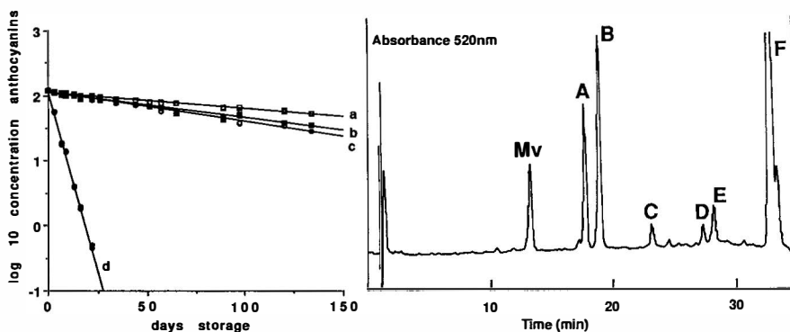
Fig. 1 (left): Logarithmic changes in malvidin 3-glucoside concentration in model wine systems. a: control, b: anthocyanins+catechin, c: anthocyanins+catechin+ferric ions, d: anthocyanins+catechin+acetaldehyde. The following equations were calculated using stepwise linear regression; the standard error is shown in brackets and the Multiple R is given at the end of the equation:
